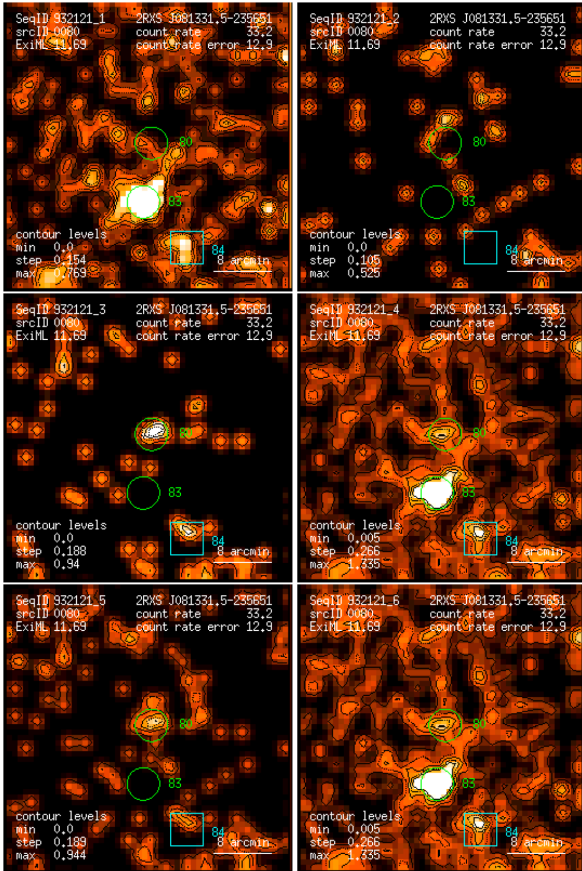
Figure 80: RASS 932121: detection 0080: band rate images, Gaussian filter: (1) PSPC channels 11 – 41, (2) 52 – 90, (3) 91 – 201, (4) 11 – 235, (5) 52 – 201, (6) 11 – 201. Broad band rates in counts/ks. Band rate contour levels in counts/ks/arcmin 2 .
