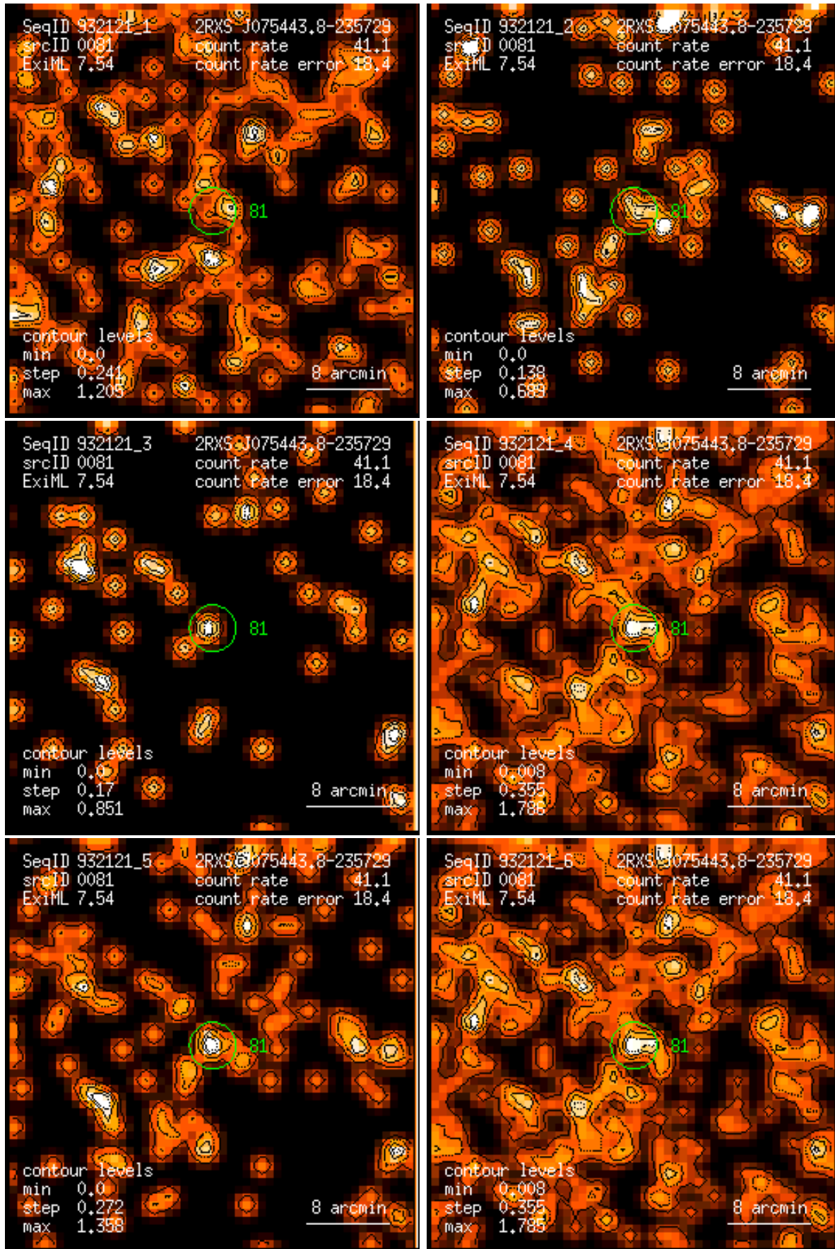
Figure 81: RASS 932121: detection 0081: band rate images, Gaussian filter: (1) PSPC channels 11 – 41, (2) 52 – 90, (3) 91 – 201, (4) 11 – 235, (5) 52 – 201, (6) 11 – 201. Broad band rates in counts/ks. Band rate contour levels in counts/ks/arcmin 2 .
