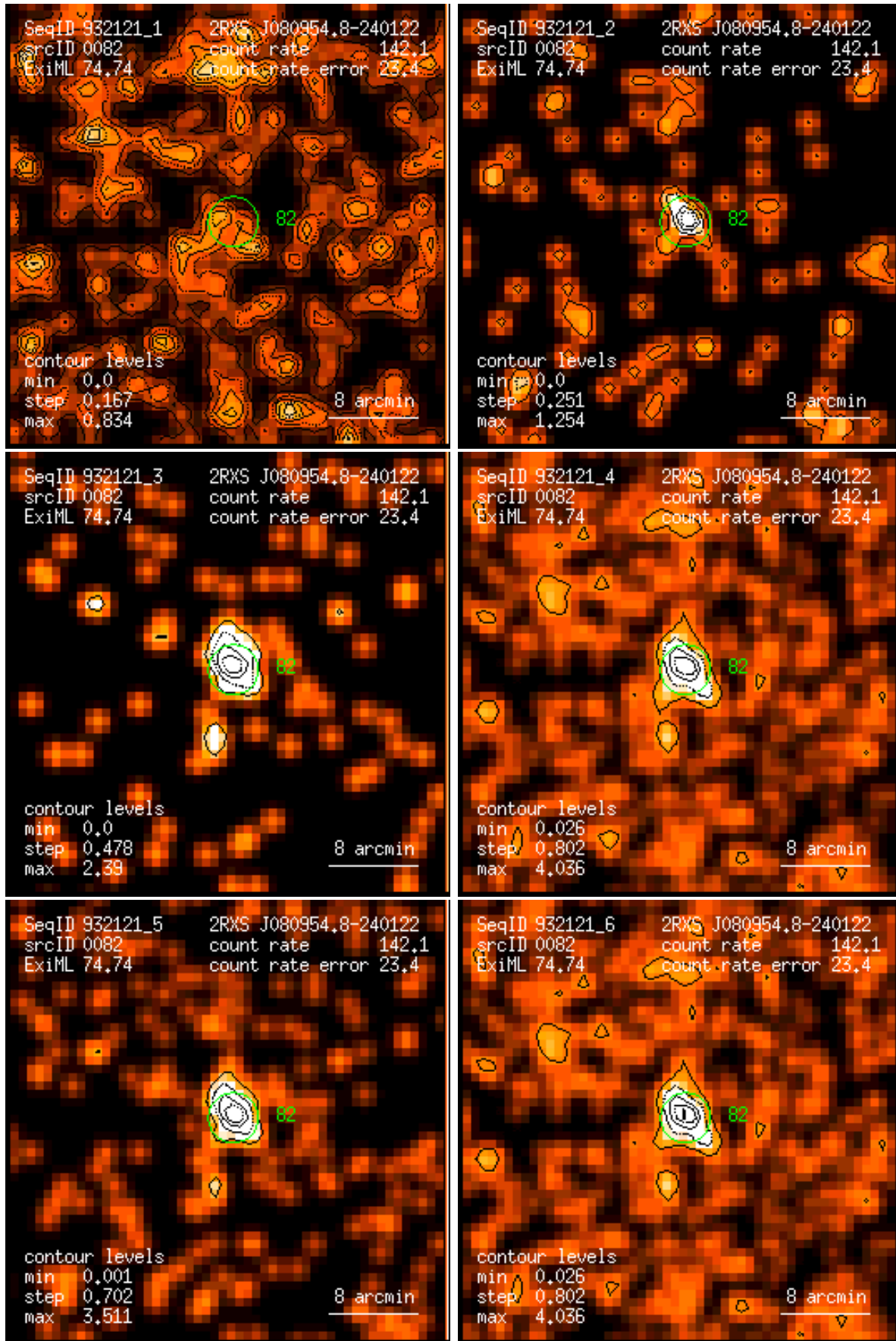
Figure 82: RASS 932121: detection 0082: band rate images, Gaussian filter: (1) PSPC channels 11 – 41, (2) 52 – 90, (3) 91 – 201, (4) 11 – 235, (5) 52 – 201, (6) 11 – 201. Broad band rates in counts/ks. Band rate contour levels in counts/ks/arcmin 2 .
