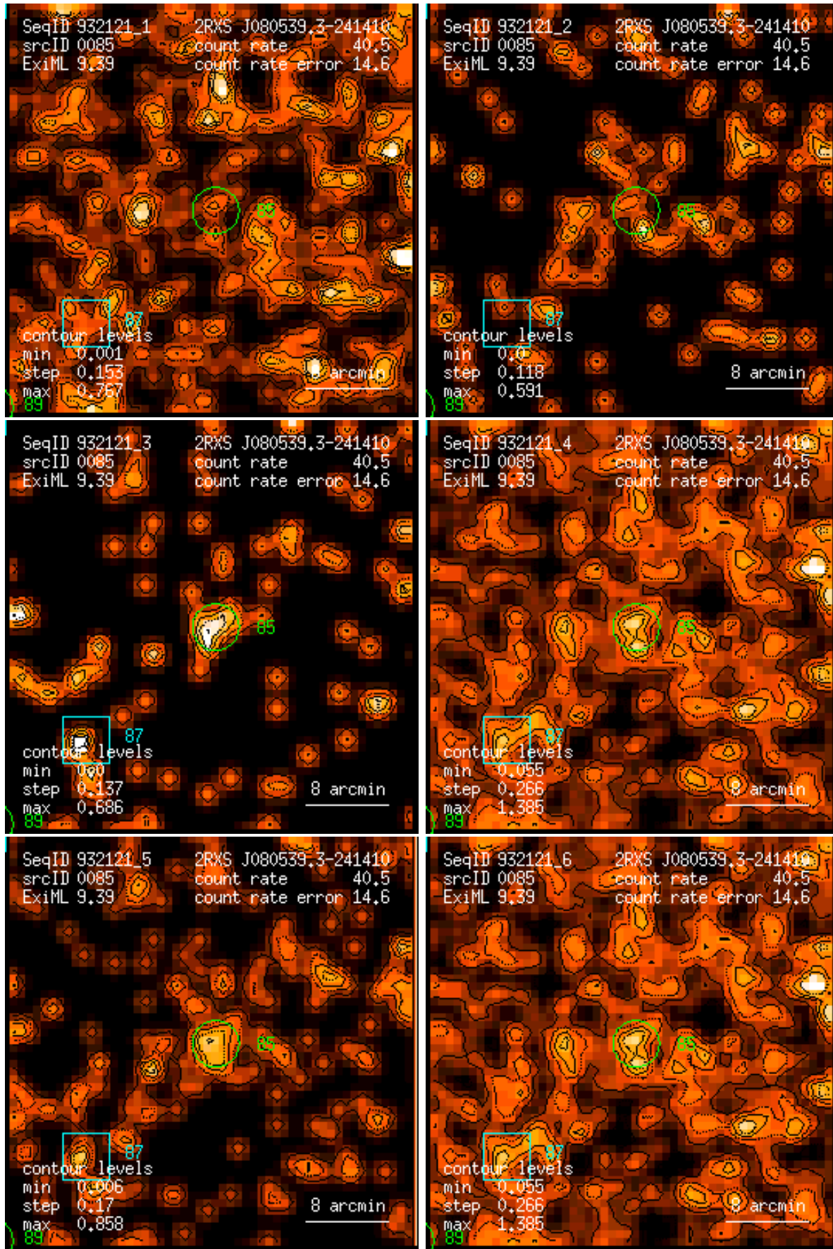
Figure 85: RASS 932121: detection 0085: band rate images, Gaussian filter: (1) PSPC channels 11 – 41, (2) 52 – 90, (3) 91 – 201, (4) 11 – 235, (5) 52 – 201, (6) 11 – 201. Broad band rates in counts/ks. Band rate contour levels in counts/ks/arcmin 2 .
