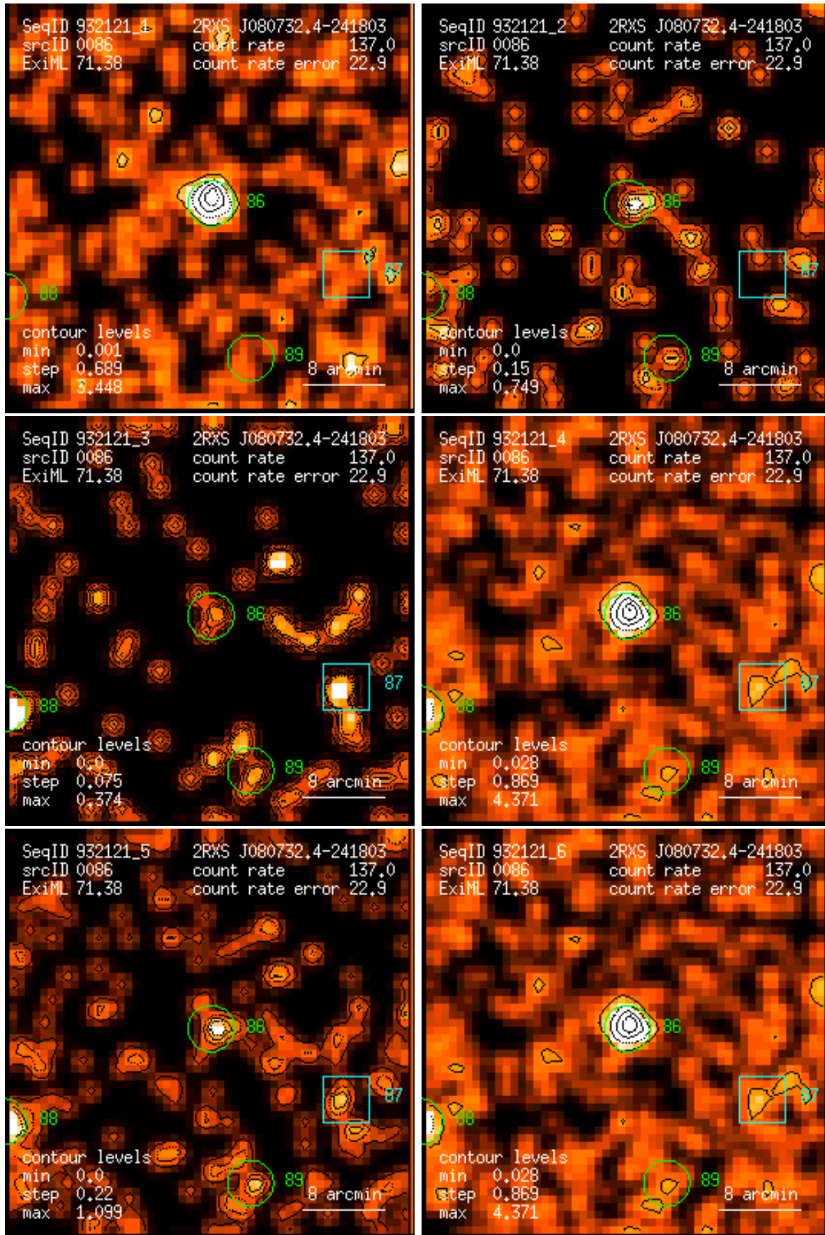
Figure 86: RASS 932121: detection 0086: band rate images, Gaussian filter: (1) PSPC channels 11 – 41, (2) 52 – 90, (3) 91 – 201, (4) 11 – 235, (5) 52 – 201, (6) 11 – 201. Broad band rates in counts/ks. Band rate contour levels in counts/ks/arcmin 2 .
