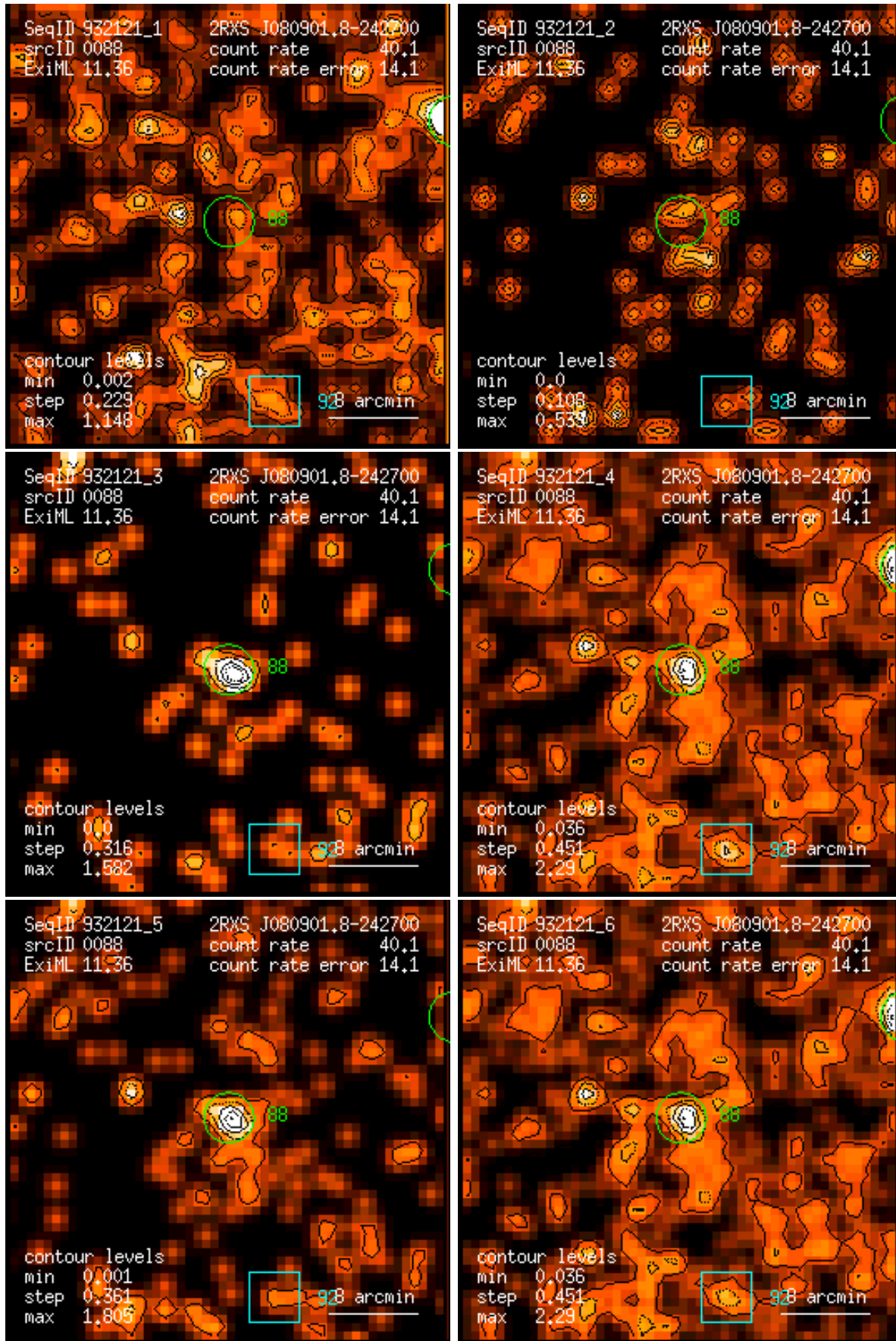
Figure 88: RASS 932121: detection 0088: band rate images, Gaussian filter: (1) PSPC channels 11 – 41, (2) 52 – 90, (3) 91 – 201, (4) 11 – 235, (5) 52 – 201, (6) 11 – 201. Broad band rates in counts/ks. Band rate contour levels in counts/ks/arcmin 2 .
