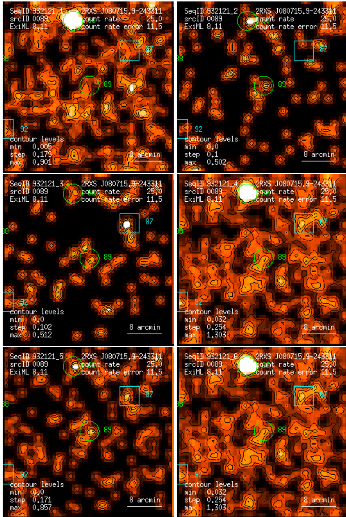
Figure 89: RASS 932121: detection 0089: band rate images, Gaussian filter: (1) PSPC channels 11 – 41, (2) 52 – 90, (3) 91 – 201, (4) 11 – 235, (5) 52 – 201, (6) 11 – 201. Broad band rates in counts/ks. Band rate contour levels in counts/ks/arcmin 2 .
