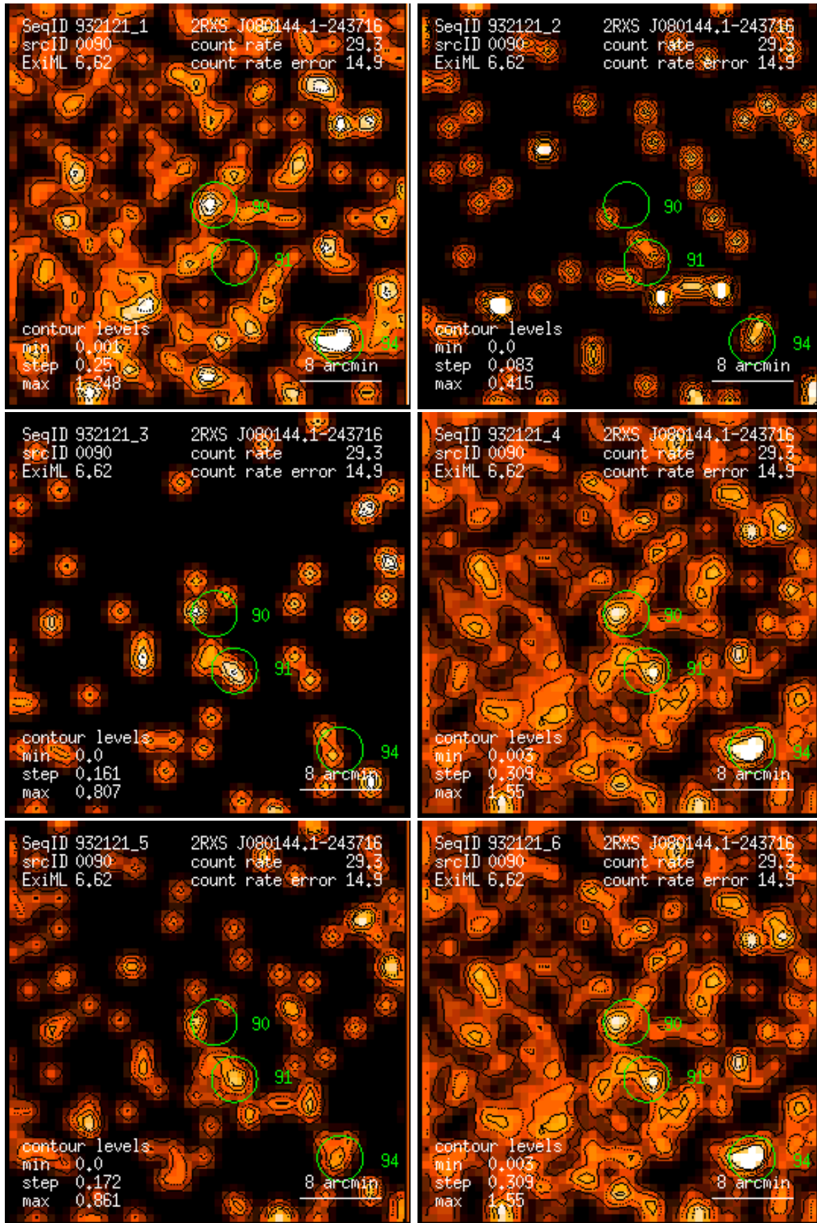
Figure 90: RASS 932121: detection 0090: band rate images, Gaussian filter: (1) PSPC channels 11 – 41, (2) 52 – 90, (3) 91 – 201, (4) 11 – 235, (5) 52 – 201, (6) 11 – 201. Broad band rates in counts/ks. Band rate contour levels in counts/ks/arcmin 2 .
