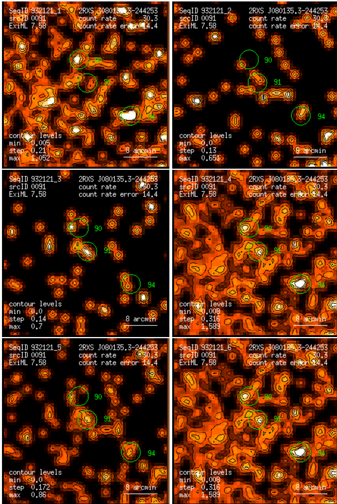
Figure 91: RASS 932121: detection 0091: band rate images, Gaussian filter: (1) PSPC channels 11 – 41, (2) 52 – 90, (3) 91 – 201, (4) 11 – 235, (5) 52 – 201, (6) 11 – 201. Broad band rates in counts/ks. Band rate contour levels in counts/ks/arcmin 2 .
