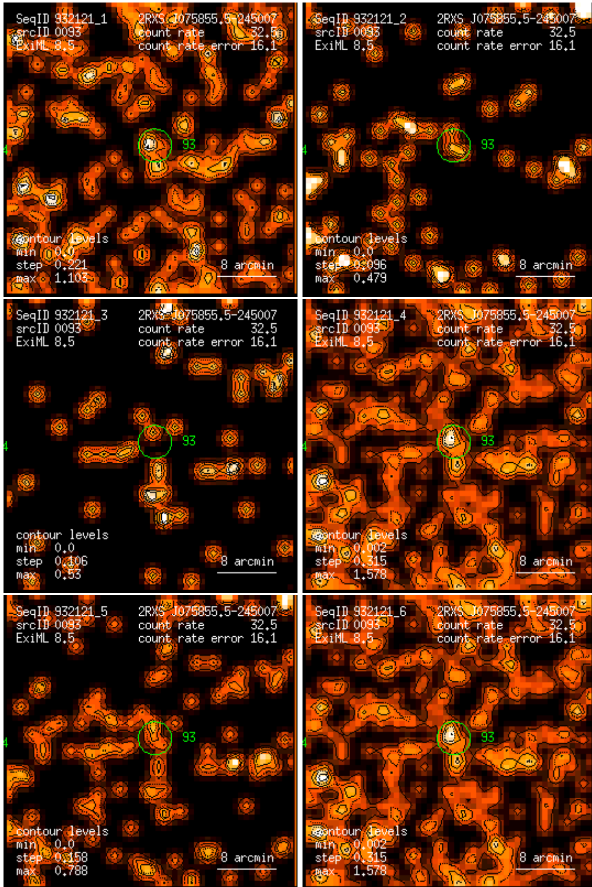
Figure 93: RASS 932121: detection 0093: band rate images, Gaussian filter: (1) PSPC channels 11 – 41, (2) 52 – 90, (3) 91 – 201, (4) 11 – 235, (5) 52 – 201, (6) 11 – 201. Broad band rates in counts/ks. Band rate contour levels in counts/ks/arcmin 2 .
