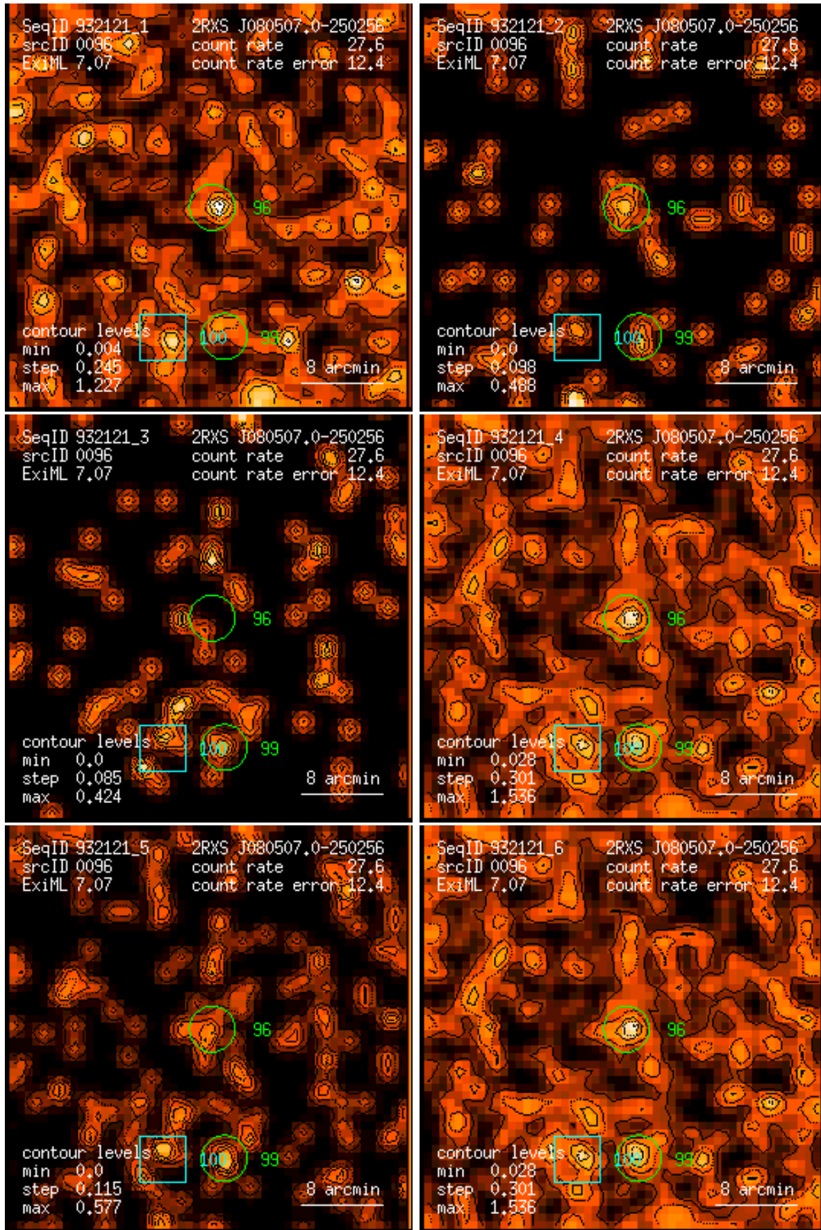
Figure 96: RASS 932121: detection 0096: band rate images, Gaussian filter: (1) PSPC channels 11 – 41, (2) 52 – 90, (3) 91 – 201, (4) 11 – 235, (5) 52 – 201, (6) 11 – 201. Broad band rates in counts/ks. Band rate contour levels in counts/ks/arcmin 2 .
