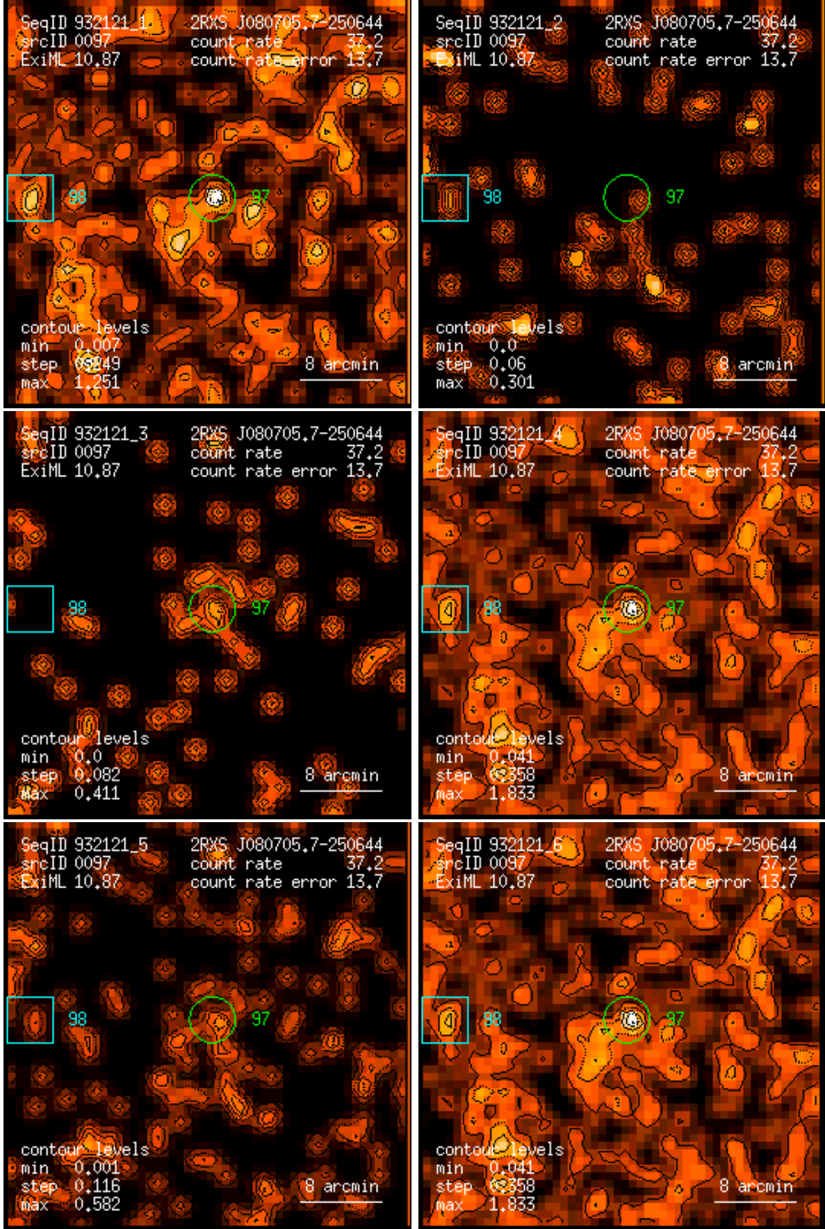
Figure 97: RASS 932121: detection 0097: band rate images, Gaussian filter: (1) PSPC channels 11 – 41, (2) 52 – 90, (3) 91 – 201, (4) 11 – 235, (5) 52 – 201, (6) 11 – 201. Broad band rates in counts/ks. Band rate contour levels in counts/ks/arcmin 2 .
