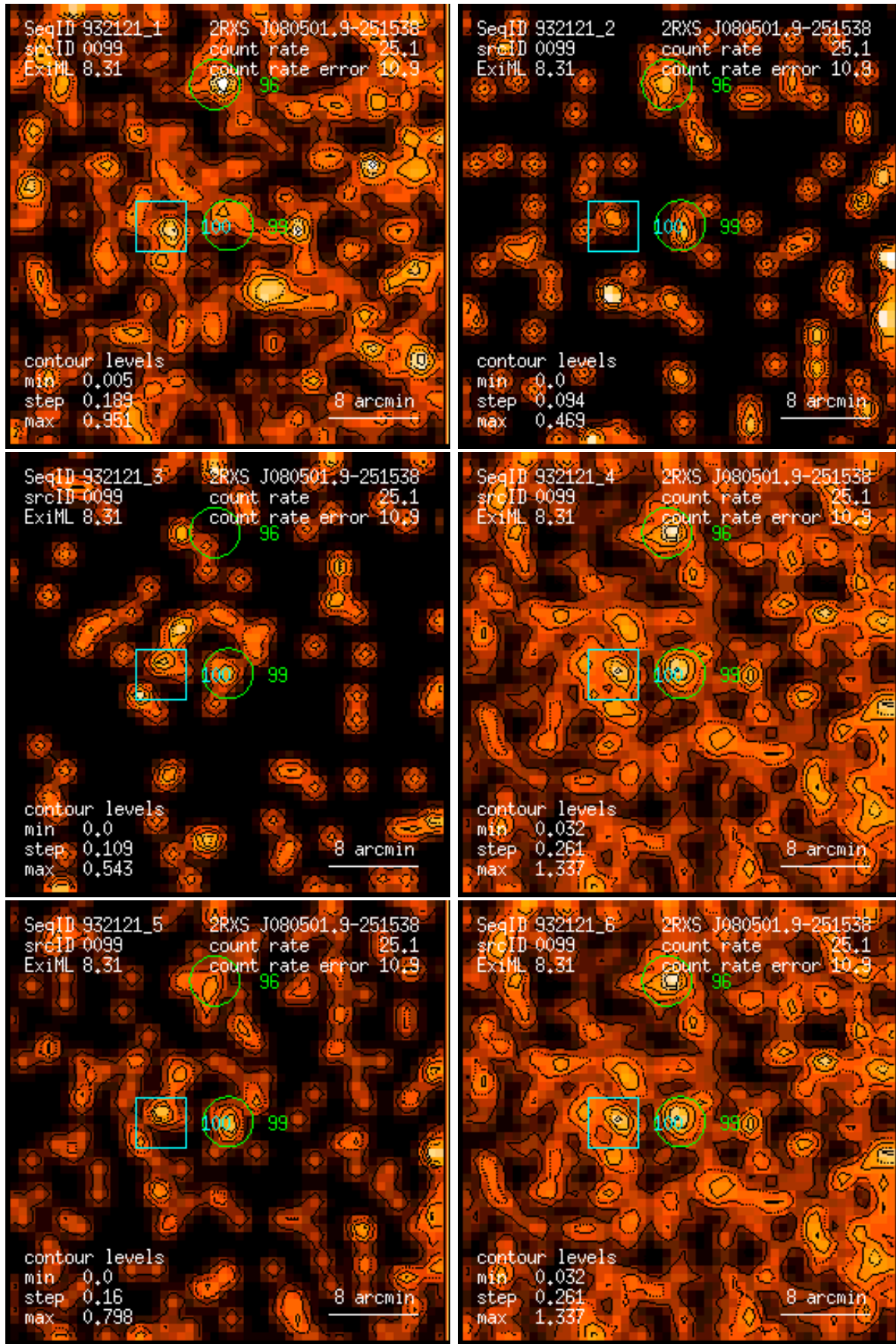
Figure 99: RASS 932121: detection 0099: band rate images, Gaussian filter: (1) PSPC channels 11 – 41, (2) 52 – 90, (3) 91 – 201, (4) 11 – 235, (5) 52 – 201, (6) 11 – 201. Broad band rates in counts/ks. Band rate contour levels in counts/ks/arcmin 2 .
