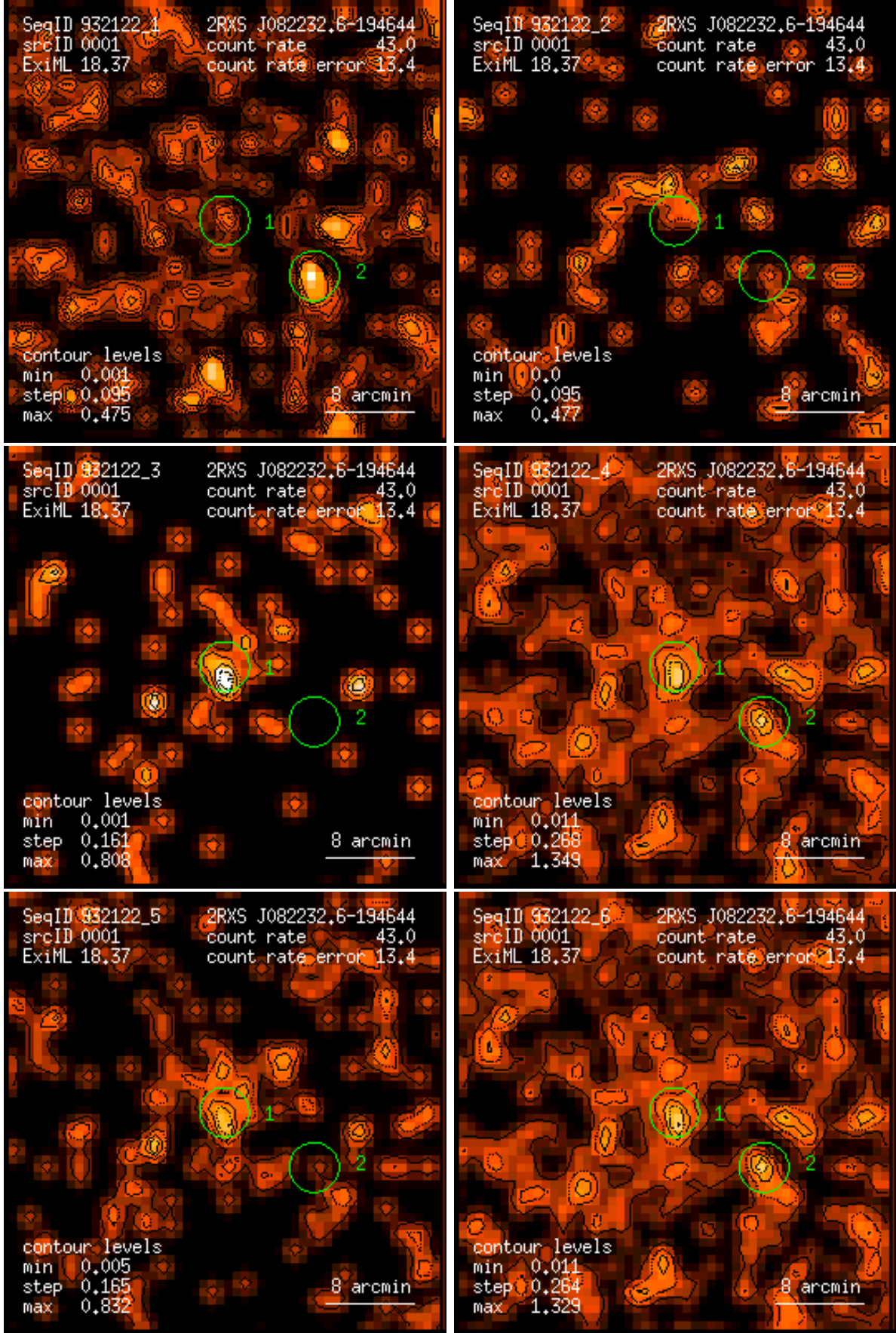
Figure 1: RASS 932122: detection 0001: band rate images, Gaussian filter: (1) PSPC channels 11 – 41, (2) 52 – 90, (3) 91 – 201, (4) 11 – 235, (5) 52 – 201, (6) 11 – 201. Broad band rates in counts/ks. Band rate contour levels in counts/ks/arcmin 2 .
