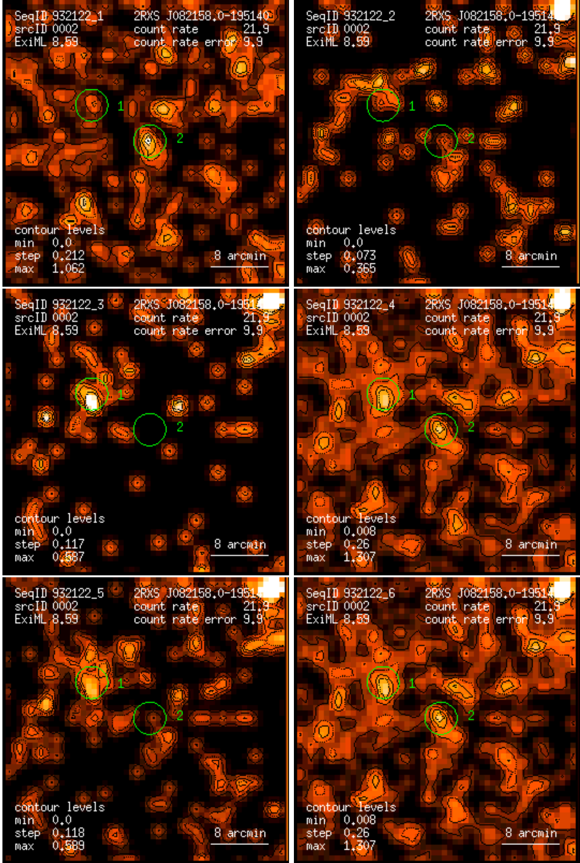
Figure 2: RASS 932122: detection 0002: band rate images, Gaussian filter: (1) PSPC channels 11 – 41, (2) 52 – 90, (3) 91 – 201, (4) 11 – 235, (5) 52 – 201, (6) 11 – 201. Broad band rates in counts/ks. Band rate contour levels in counts/ks/arcmin 2 .
