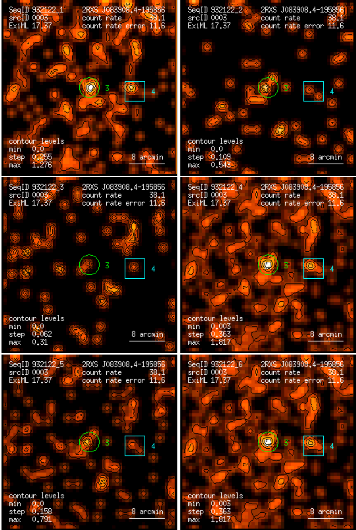
Figure 3: RASS 932122: detection 0003: band rate images, Gaussian filter: (1) PSPC channels 11 – 41, (2) 52 – 90, (3) 91 – 201, (4) 11 – 235, (5) 52 – 201, (6) 11 – 201. Broad band rates in counts/ks. Band rate contour levels in counts/ks/arcmin 2 .
