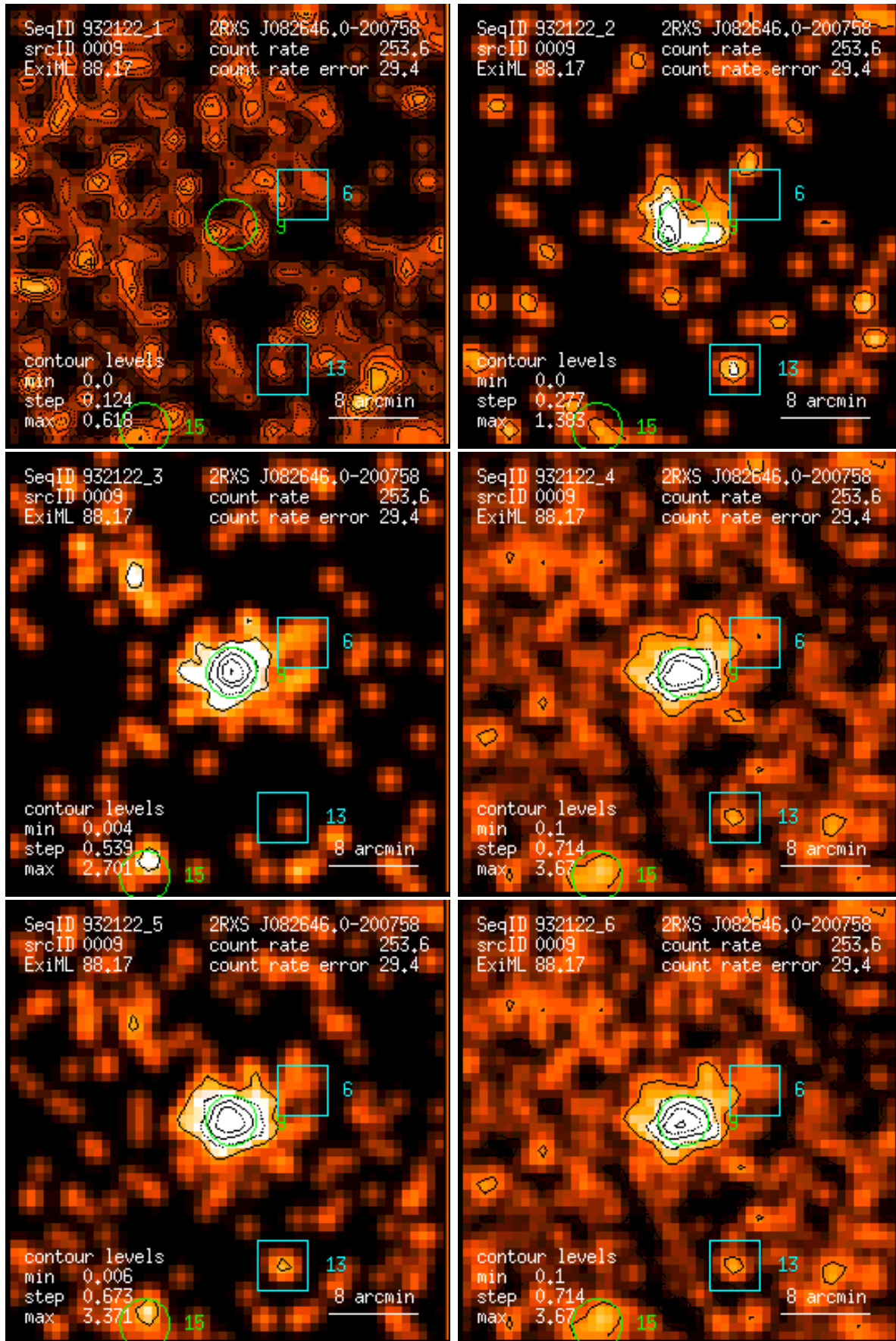
Figure 9: RASS 932122: detection 0009: band rate images, Gaussian filter: (1) PSPC channels 11 – 41, (2) 52 – 90, (3) 91 – 201, (4) 11 – 235, (5) 52 – 201, (6) 11 – 201. Broad band rates in counts/ks. Band rate contour levels in counts/ks/arcmin 2 .
