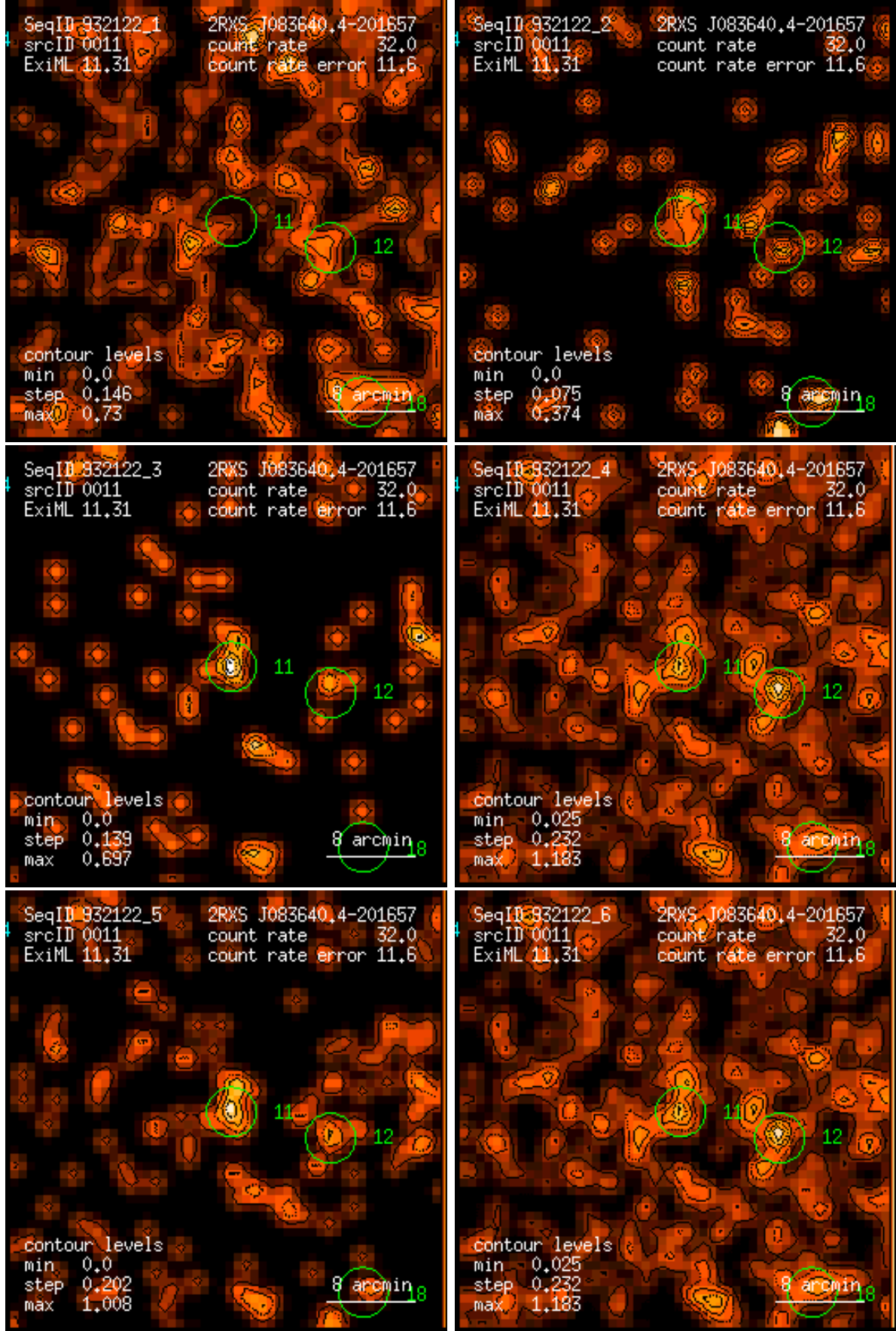
Figure 11: RASS 932122: detection 0011: band rate images, Gaussian filter: (1) PSPC channels 11 – 41, (2) 52 – 90, (3) 91 – 201, (4) 11 – 235, (5) 52 – 201, (6) 11 – 201. Broad band rates in counts/ks. Band rate contour levels in counts/ks/arcmin 2 .
