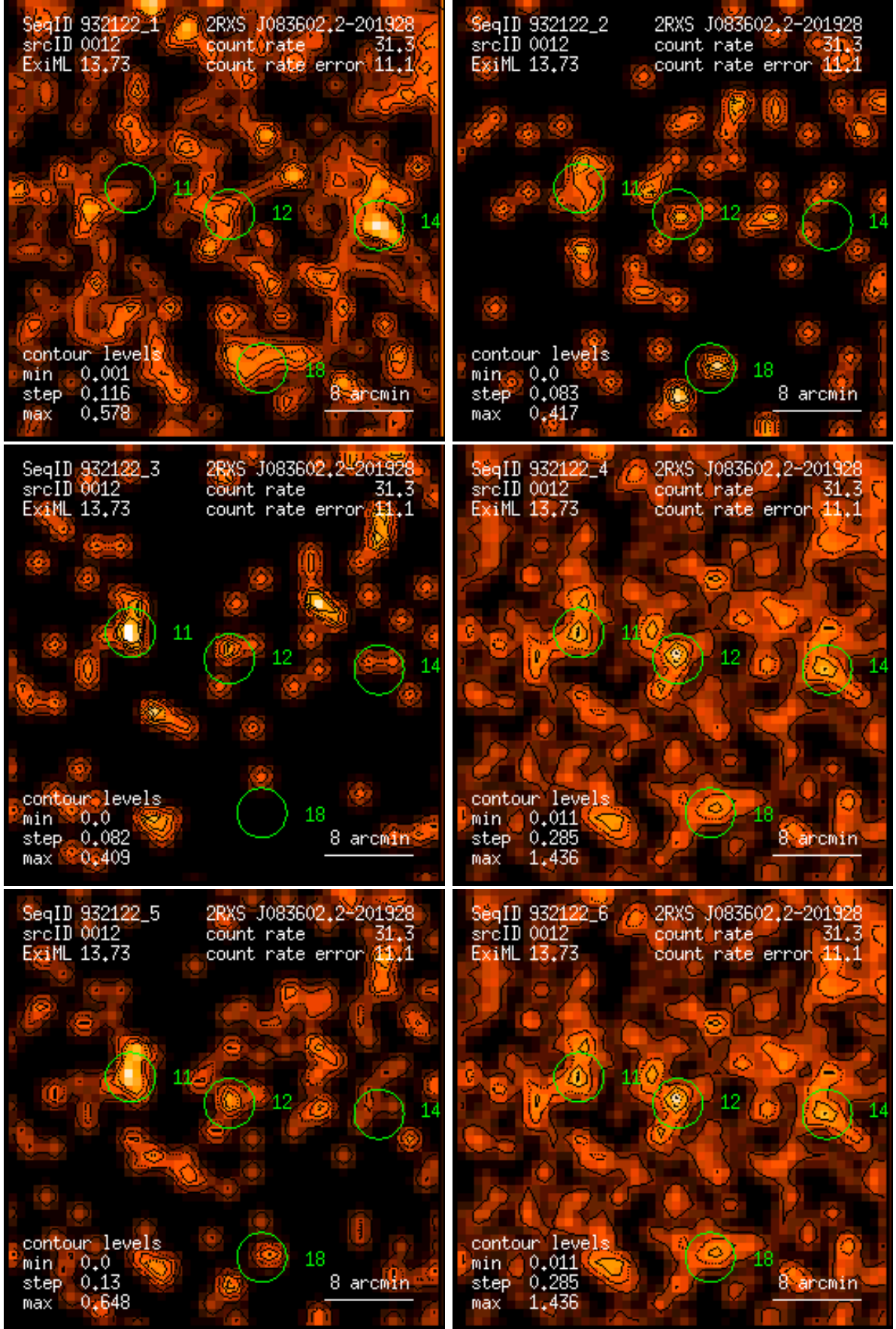
Figure 12: RASS 932122: detection 0012: band rate images, Gaussian filter: (1) PSPC channels 11 – 41, (2) 52 – 90, (3) 91 – 201, (4) 11 – 235, (5) 52 – 201, (6) 11 – 201. Broad band rates in counts/ks. Band rate contour levels in counts/ks/arcmin 2 .
