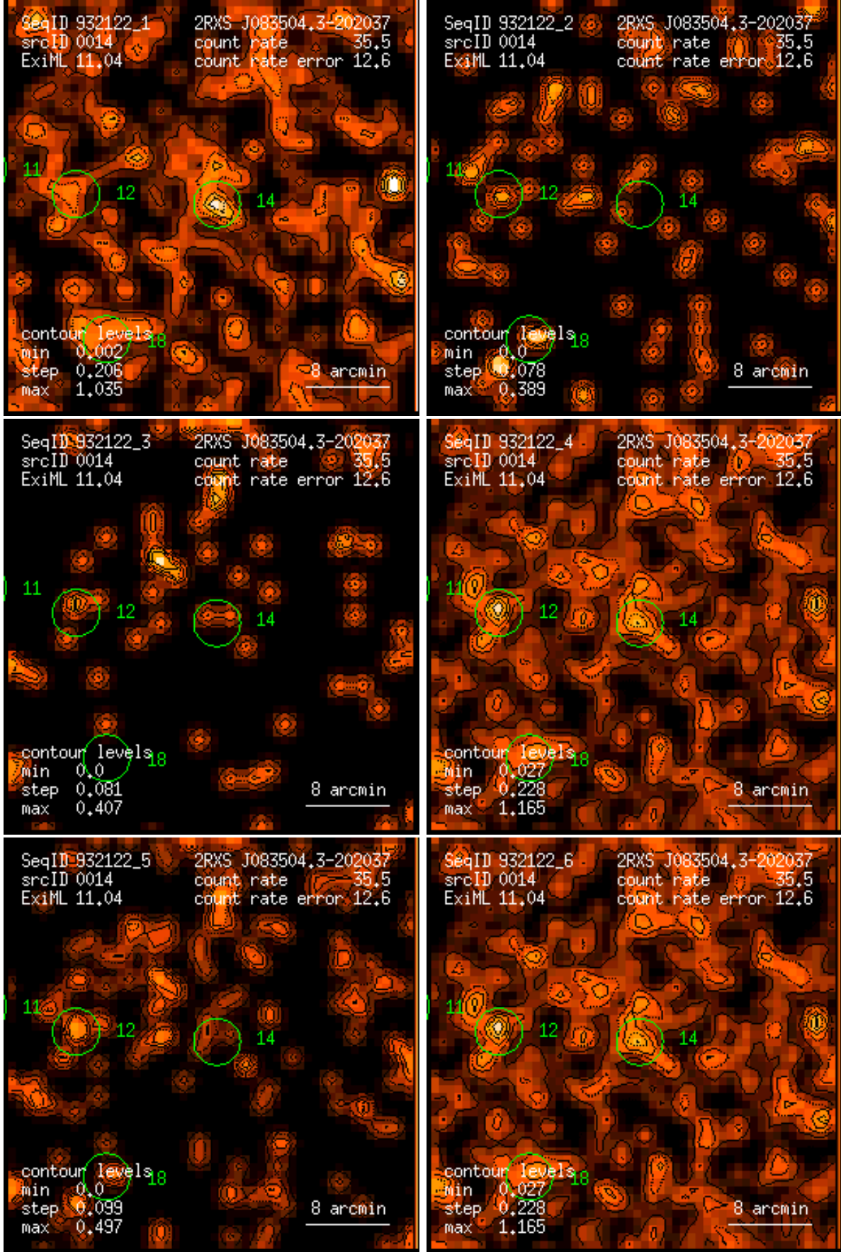
Figure 14: RASS 932122: detection 0014: band rate images, Gaussian filter: (1) PSPC channels 11 – 41, (2) 52 – 90, (3) 91 – 201, (4) 11 – 235, (5) 52 – 201, (6) 11 – 201. Broad band rates in counts/ks. Band rate contour levels in counts/ks/arcmin 2 .
