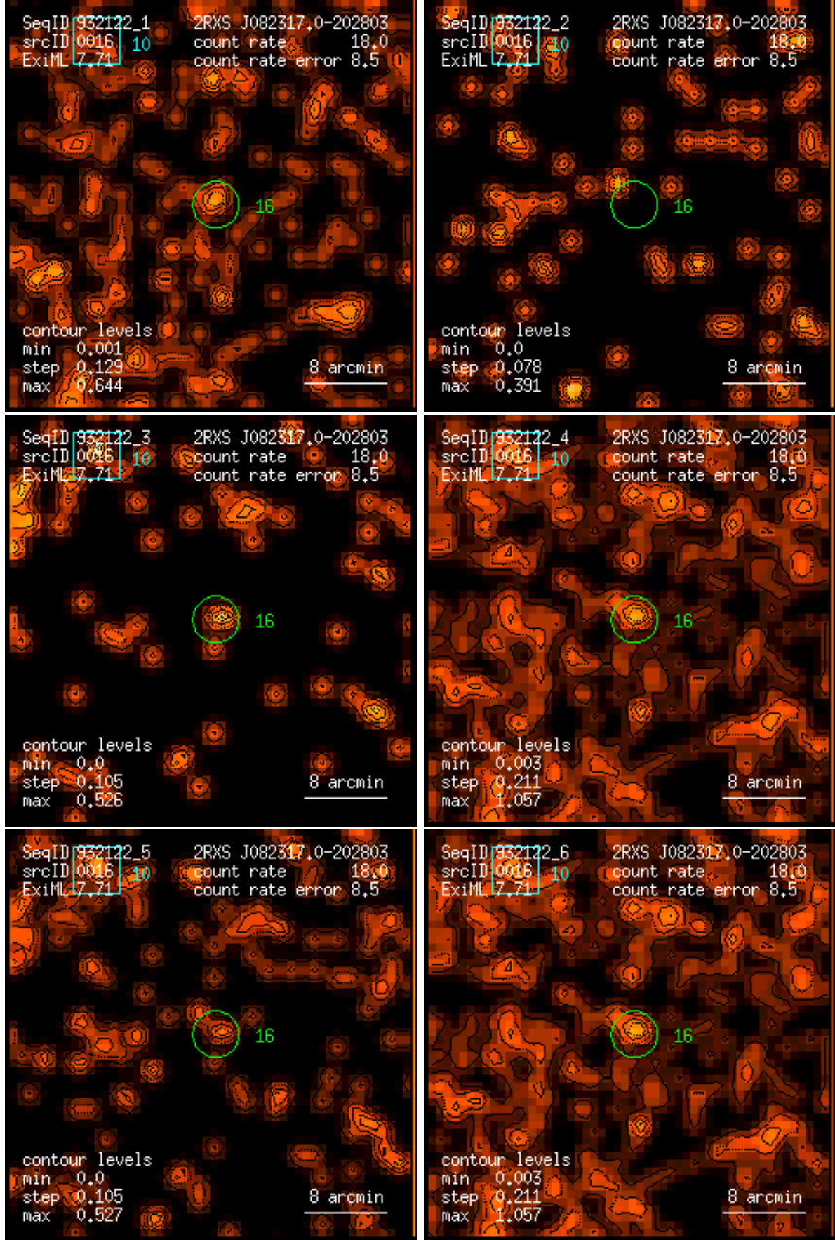
Figure 16: RASS 932122: detection 0016: band rate images, Gaussian filter: (1) PSPC channels 11 – 41, (2) 52 – 90, (3) 91 – 201, (4) 11 – 235, (5) 52 – 201, (6) 11 – 201. Broad band rates in counts/ks. Band rate contour levels in counts/ks/arcmin 2 .
