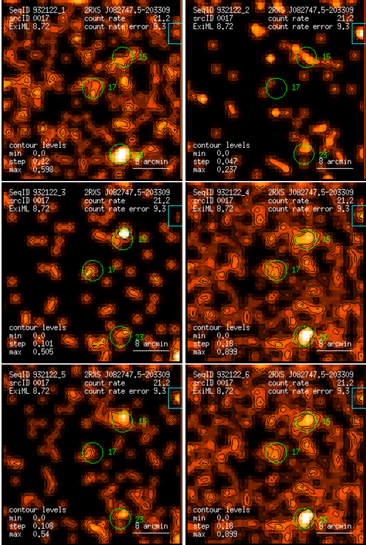
Figure 17: RASS 932122: detection 0017: band rate images, Gaussian filter: (1) PSPC channels 11 – 41, (2) 52 – 90, (3) 91 – 201, (4) 11 – 235, (5) 52 – 201, (6) 11 – 201. Broad band rates in counts/ks. Band rate contour levels in counts/ks/arcmin 2 .
