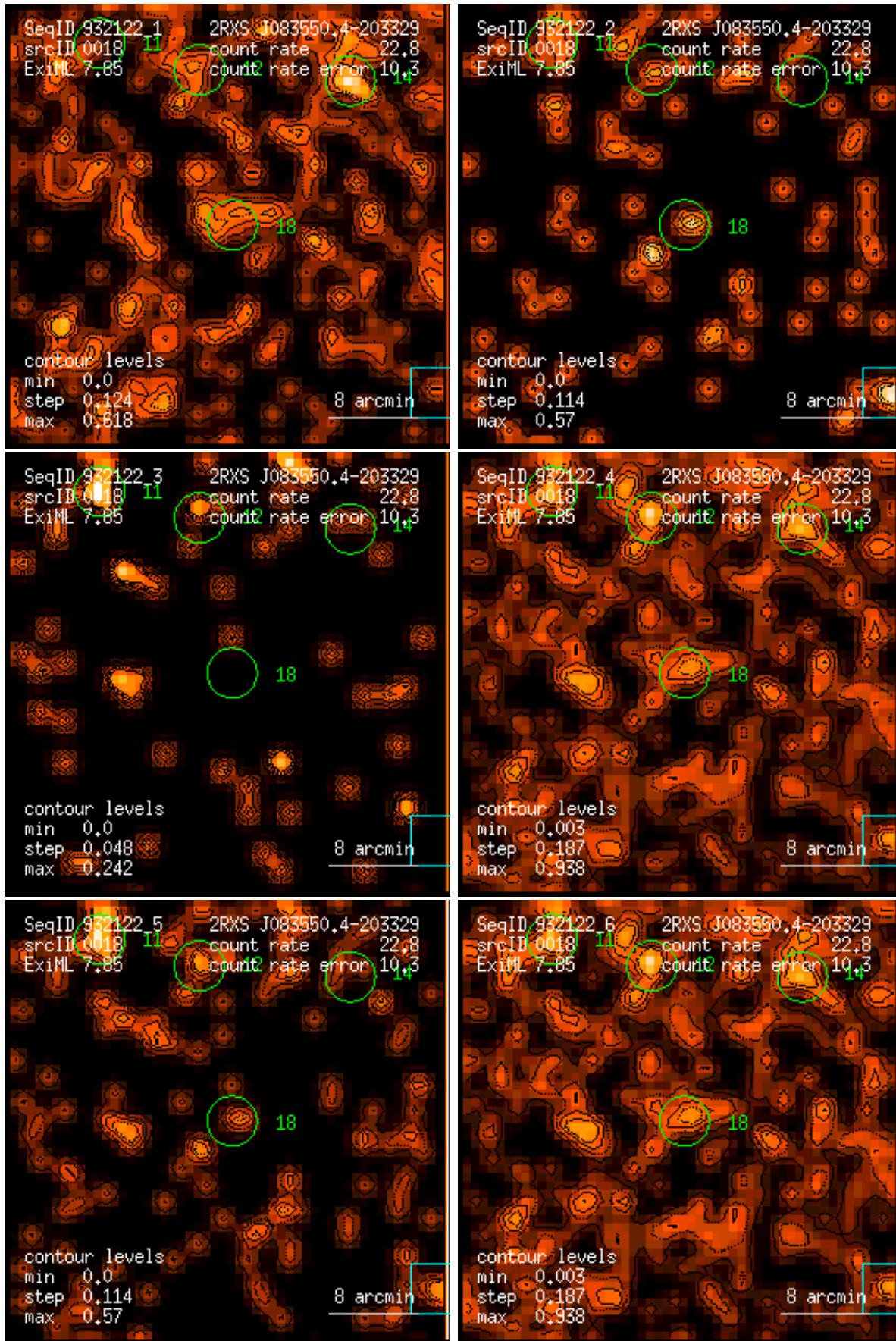
Figure 18: RASS 932122: detection 0018: band rate images, Gaussian filter: (1) PSPC channels 11 – 41, (2) 52 – 90, (3) 91 – 201, (4) 11 – 235, (5) 52 – 201, (6) 11 – 201. Broad band rates in counts/ks. Band rate contour levels in counts/ks/arcmin 2 .
