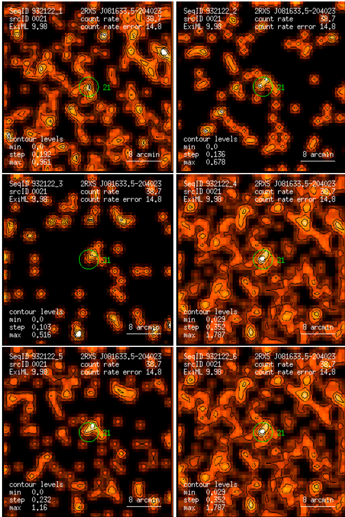
Figure 21: RASS 932122: detection 0021: band rate images, Gaussian filter: (1) PSPC channels 11 – 41, (2) 52 – 90, (3) 91 – 201, (4) 11 – 235, (5) 52 – 201, (6) 11 – 201. Broad band rates in counts/ks. Band rate contour levels in counts/ks/arcmin 2 .
