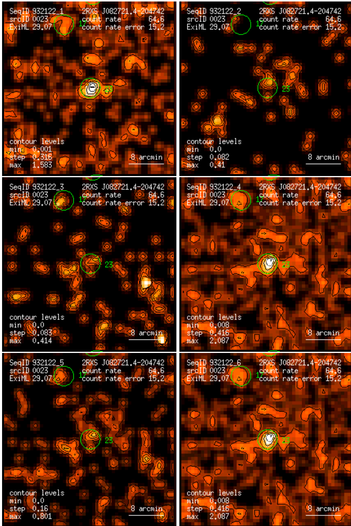
Figure 23: RASS 932122: detection 0023: band rate images, Gaussian filter: (1) PSPC channels 11 – 41, (2) 52 – 90, (3) 91 – 201, (4) 11 – 235, (5) 52 – 201, (6) 11 – 201. Broad band rates in counts/ks. Band rate contour levels in counts/ks/arcmin 2 .
