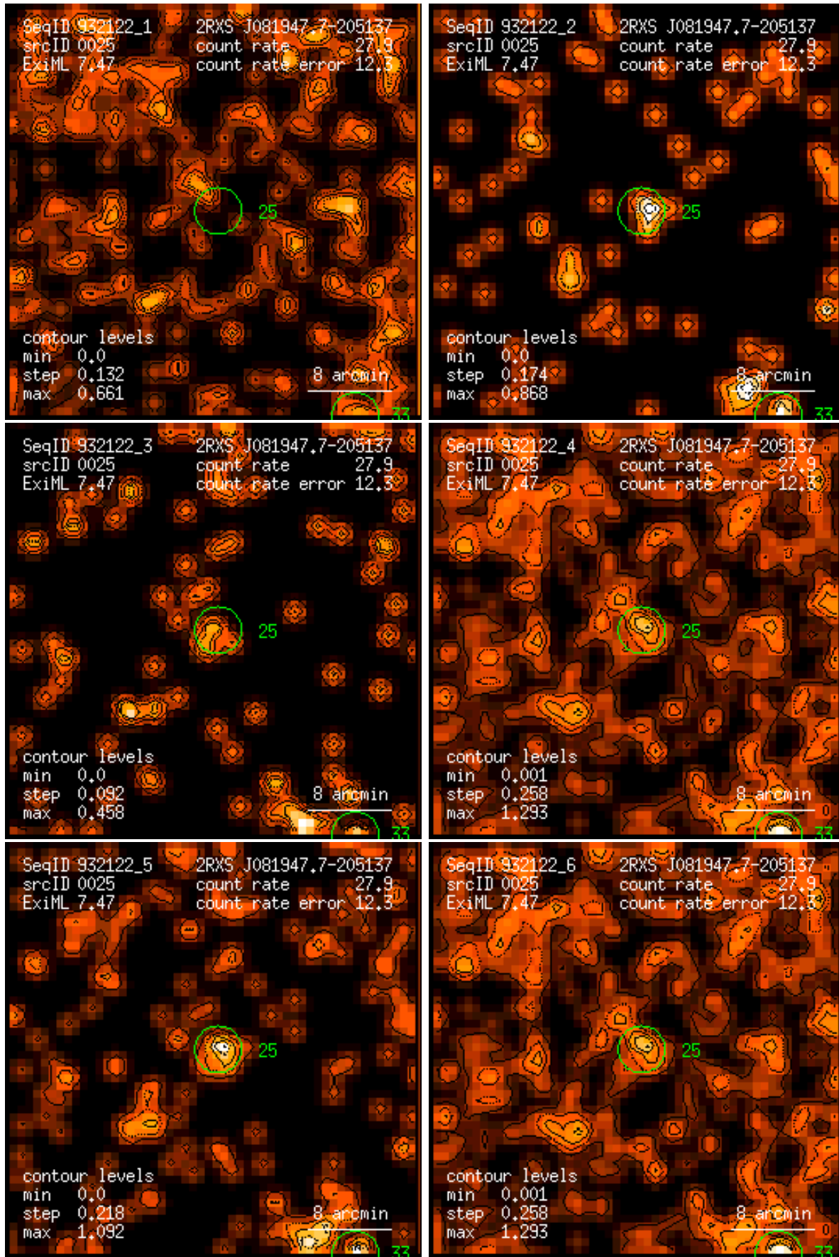
Figure 25: RASS 932122: detection 0025: band rate images, Gaussian filter: (1) PSPC channels 11 – 41, (2) 52 – 90, (3) 91 – 201, (4) 11 – 235, (5) 52 – 201, (6) 11 – 201. Broad band rates in counts/ks. Band rate contour levels in counts/ks/arcmin 2 .
