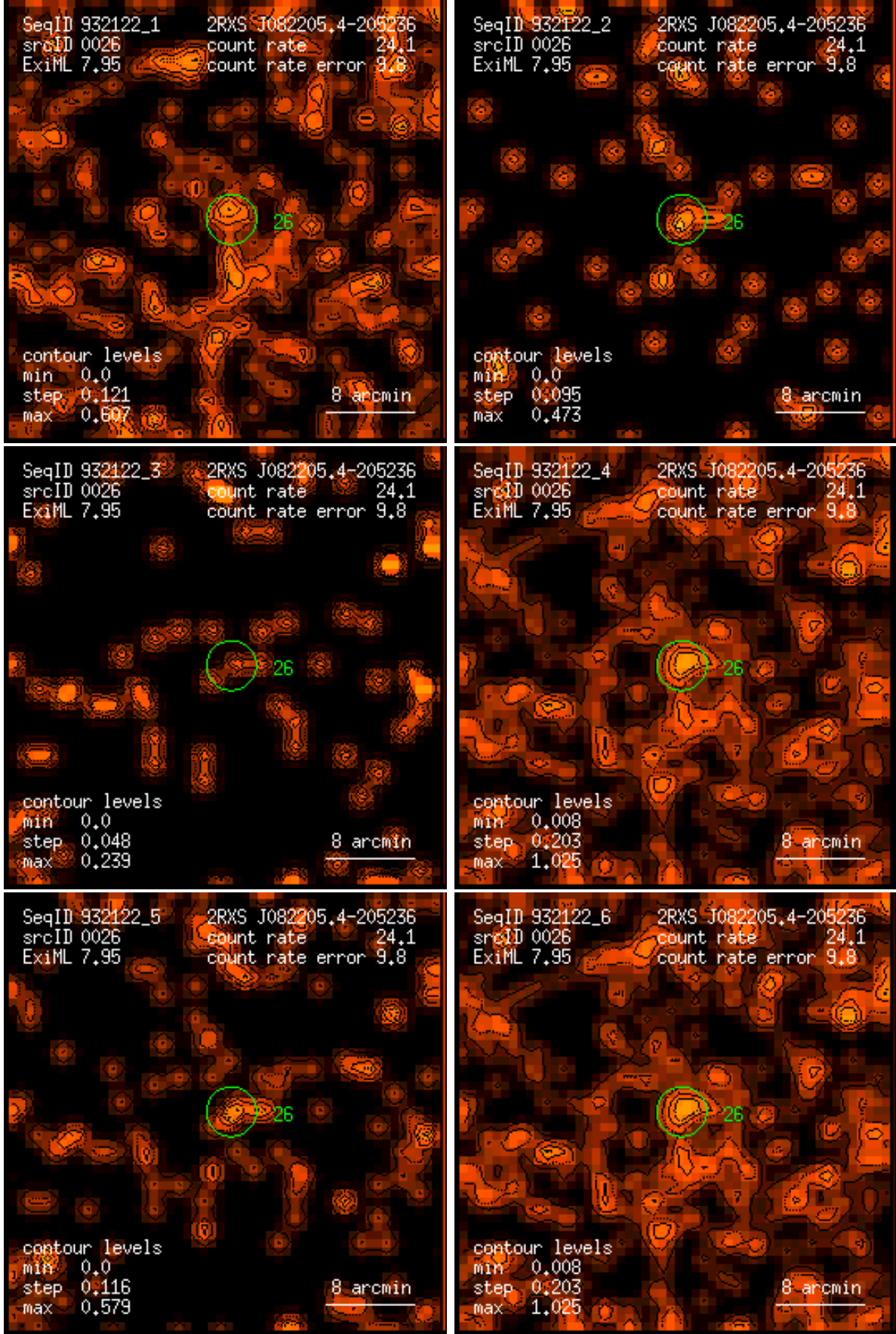
Figure 26: RASS 932122: detection 0026: band rate images, Gaussian filter: (1) PSPC channels 11 – 41, (2) 52 – 90, (3) 91 – 201, (4) 11 – 235, (5) 52 – 201, (6) 11 – 201. Broad band rates in counts/ks. Band rate contour levels in counts/ks/arcmin 2 .
