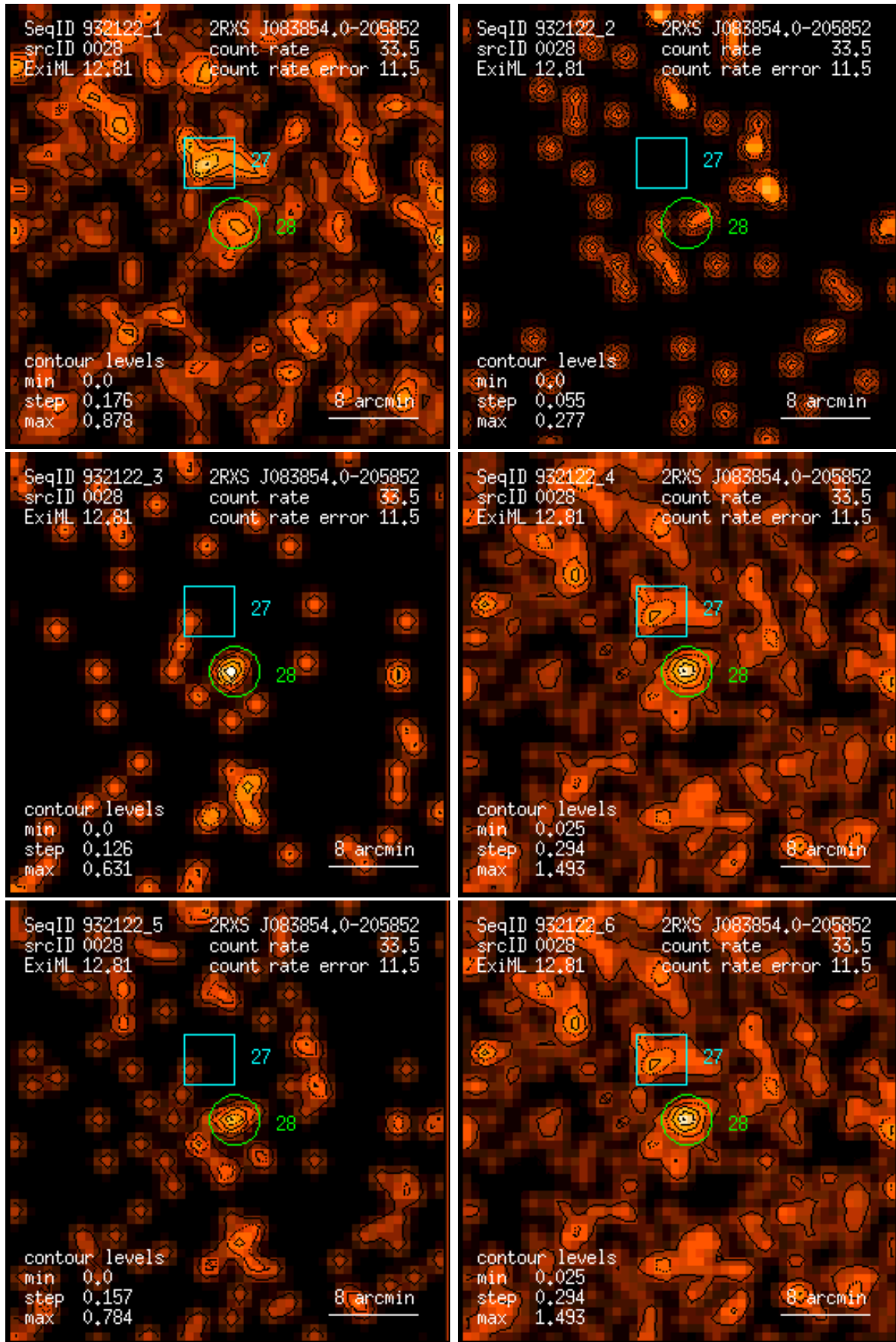
Figure 28: RASS 932122: detection 0028: band rate images, Gaussian filter: (1) PSPC channels 11 – 41, (2) 52 – 90, (3) 91 – 201, (4) 11 – 235, (5) 52 – 201, (6) 11 – 201. Broad band rates in counts/ks. Band rate contour levels in counts/ks/arcmin 2 .
