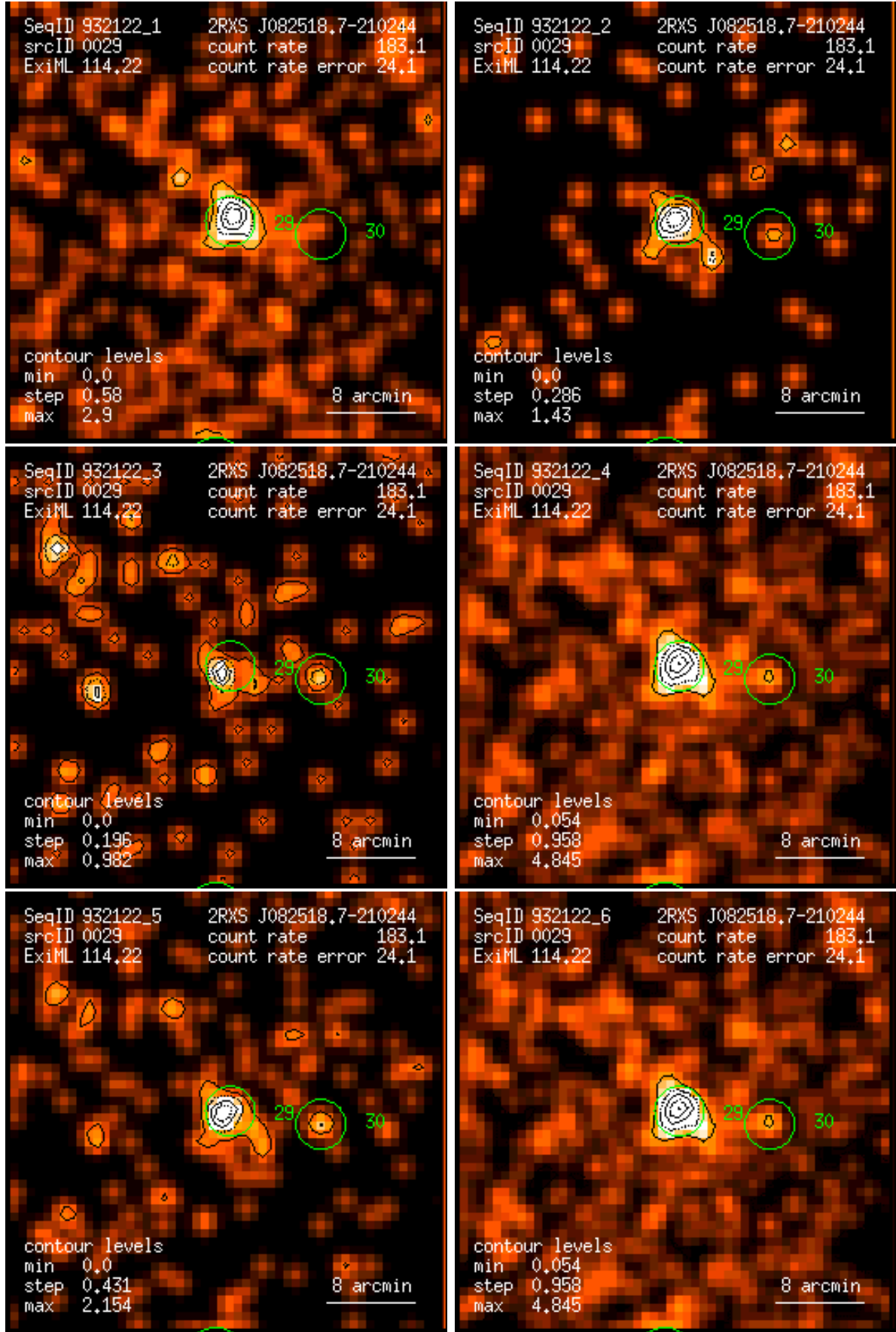
Figure 29: RASS 932122: detection 0029: band rate images, Gaussian filter: (1) PSPC channels 11 – 41, (2) 52 – 90, (3) 91 – 201, (4) 11 – 235, (5) 52 – 201, (6) 11 – 201. Broad band rates in counts/ks. Band rate contour levels in counts/ks/arcmin 2 .
