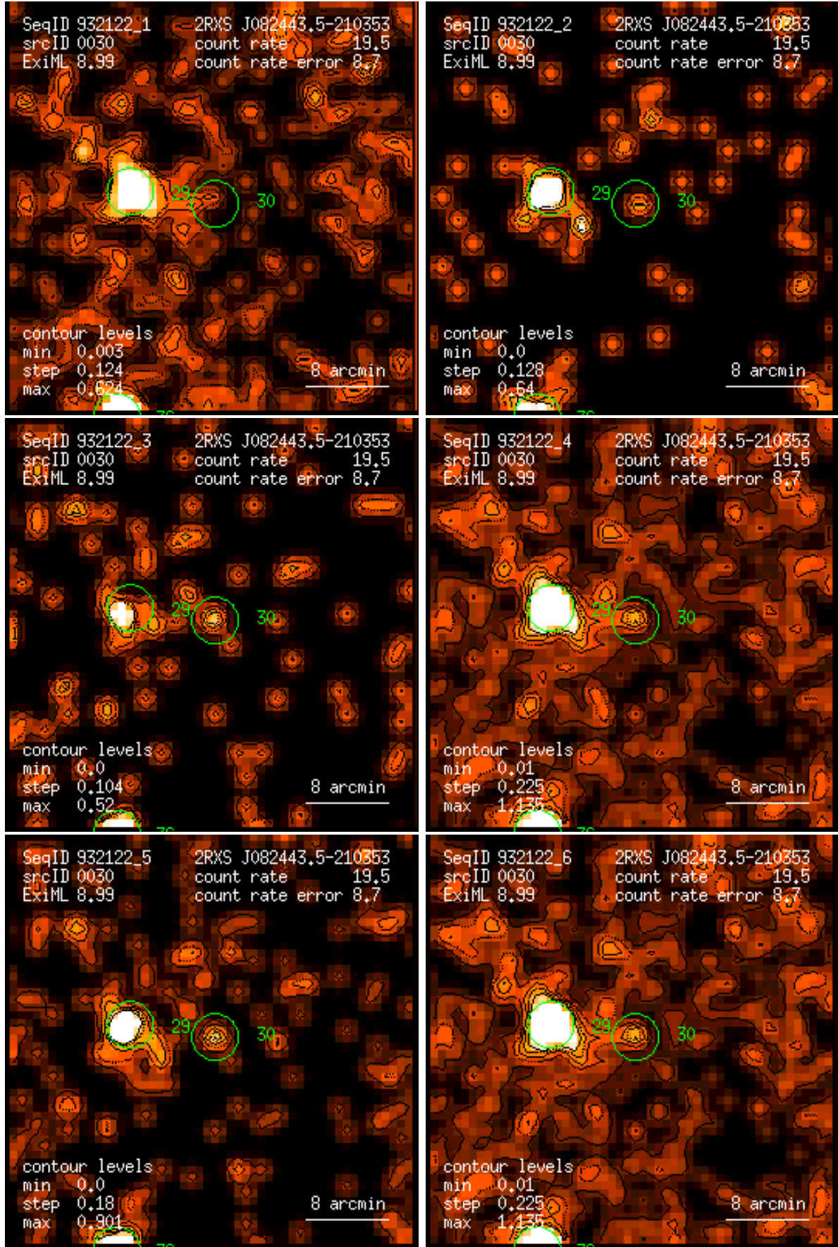
Figure 30: RASS 932122: detection 0030: band rate images, Gaussian filter: (1) PSPC channels 11 – 41, (2) 52 – 90, (3) 91 – 201, (4) 11 – 235, (5) 52 – 201, (6) 11 – 201. Broad band rates in counts/ks. Band rate contour levels in counts/ks/arcmin 2 .
