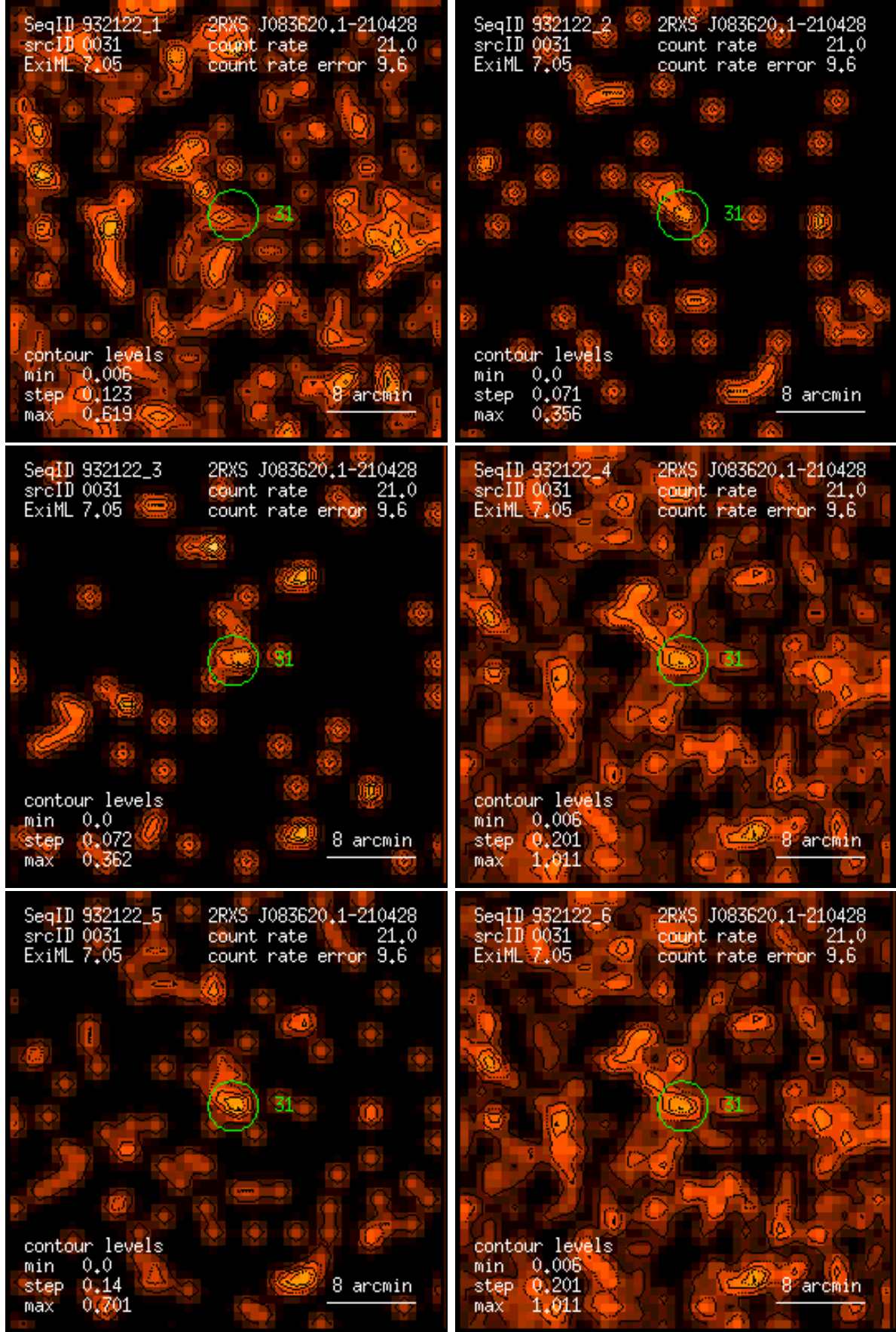
Figure 31: RASS 932122: detection 0031: band rate images, Gaussian filter: (1) PSPC channels 11 – 41, (2) 52 – 90, (3) 91 – 201, (4) 11 – 235, (5) 52 – 201, (6) 11 – 201. Broad band rates in counts/ks. Band rate contour levels in counts/ks/arcmin 2 .
