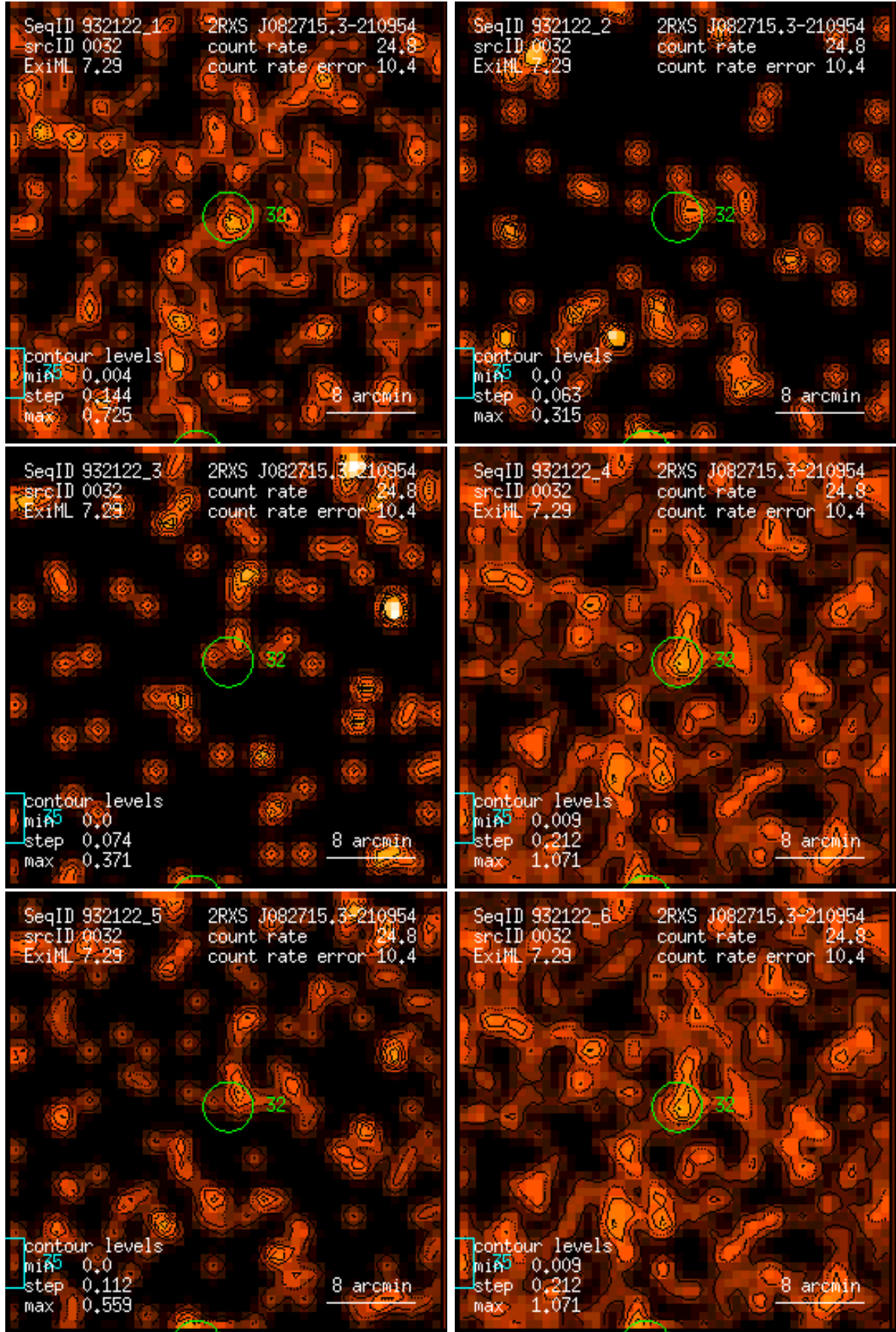
Figure 32: RASS 932122: detection 0032: band rate images, Gaussian filter: (1) PSPC channels 11 – 41, (2) 52 – 90, (3) 91 – 201, (4) 11 – 235, (5) 52 – 201, (6) 11 – 201. Broad band rates in counts/ks. Band rate contour levels in counts/ks/arcmin 2 .
