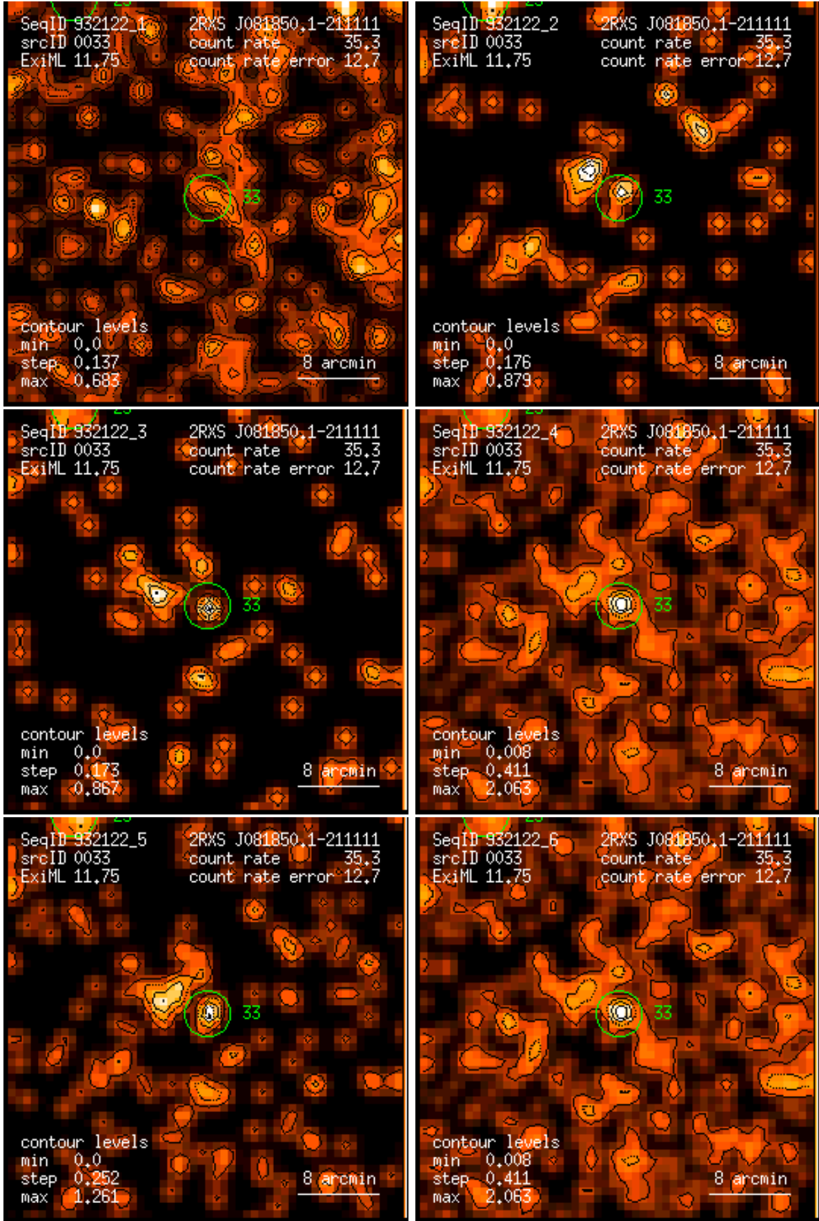
Figure 33: RASS 932122: detection 0033: band rate images, Gaussian filter: (1) PSPC channels 11 – 41, (2) 52 – 90, (3) 91 – 201, (4) 11 – 235, (5) 52 – 201, (6) 11 – 201. Broad band rates in counts/ks. Band rate contour levels in counts/ks/arcmin 2 .
