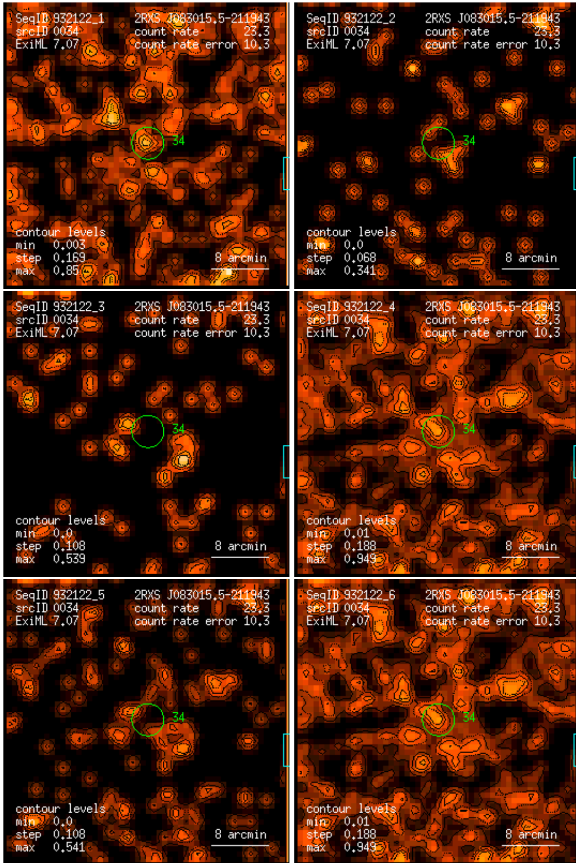
Figure 34: RASS 932122: detection 0034: band rate images, Gaussian filter: (1) PSPC channels 11 – 41, (2) 52 – 90, (3) 91 – 201, (4) 11 – 235, (5) 52 – 201, (6) 11 – 201. Broad band rates in counts/ks. Band rate contour levels in counts/ks/arcmin 2 .
