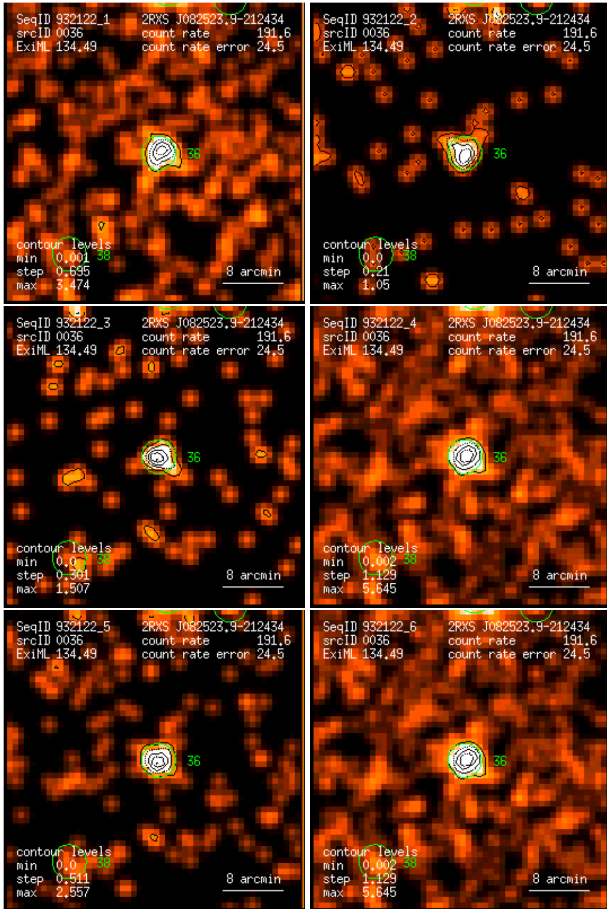
Figure 36: RASS 932122: detection 0036: band rate images, Gaussian filter: (1) PSPC channels 11 – 41, (2) 52 – 90, (3) 91 – 201, (4) 11 – 235, (5) 52 – 201, (6) 11 – 201. Broad band rates in counts/ks. Band rate contour levels in counts/ks/arcmin 2 .
