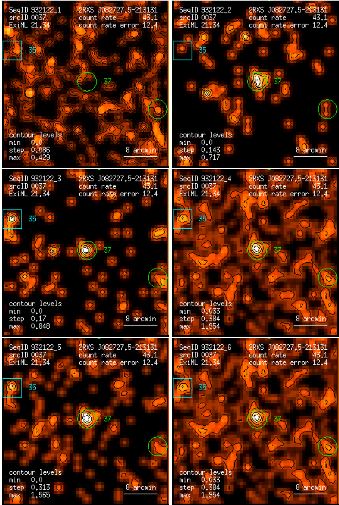
Figure 37: RASS 932122: detection 0037: band rate images, Gaussian filter: (1) PSPC channels 11 – 41, (2) 52 – 90, (3) 91 – 201, (4) 11 – 235, (5) 52 – 201, (6) 11 – 201. Broad band rates in counts/ks. Band rate contour levels in counts/ks/arcmin 2 .
