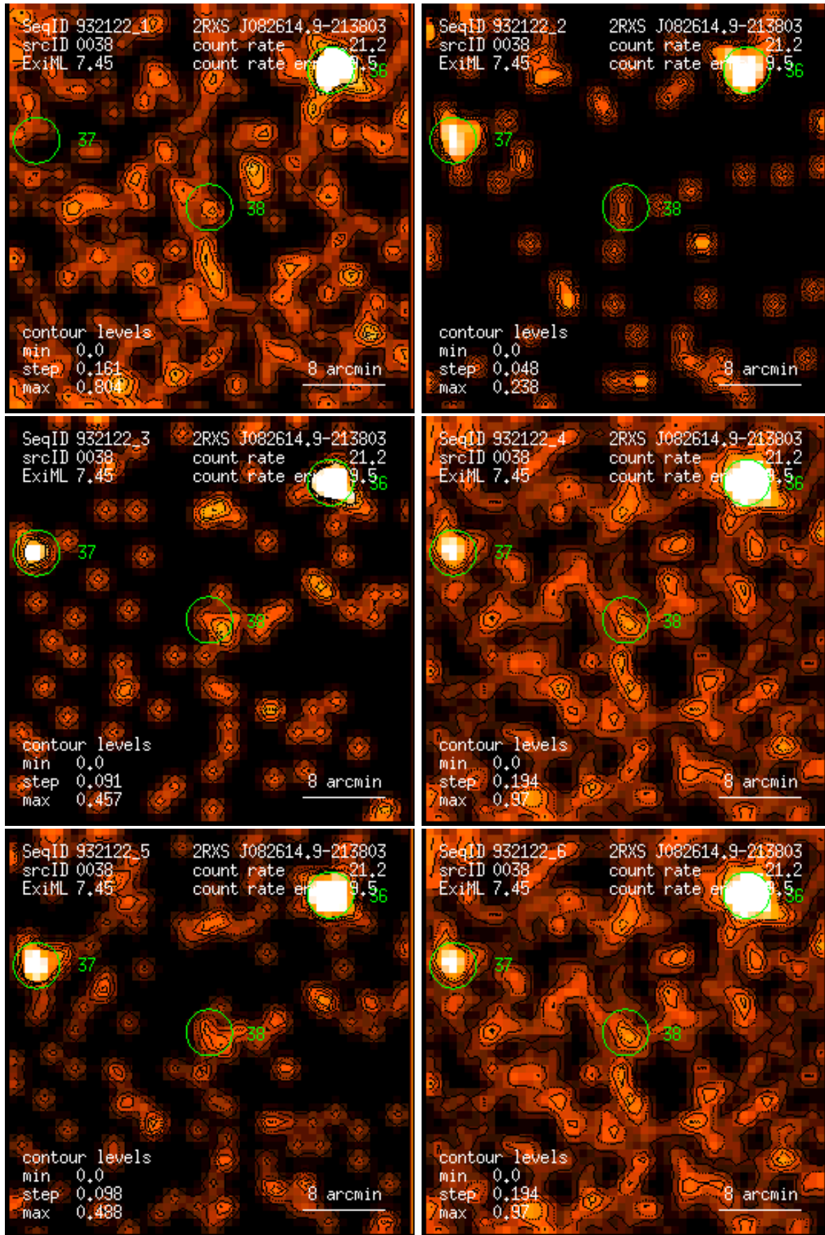
Figure 38: RASS 932122: detection 0038: band rate images, Gaussian filter: (1) PSPC channels 11 – 41, (2) 52 – 90, (3) 91 – 201, (4) 11 – 235, (5) 52 – 201, (6) 11 – 201. Broad band rates in counts/ks. Band rate contour levels in counts/ks/arcmin 2 .
