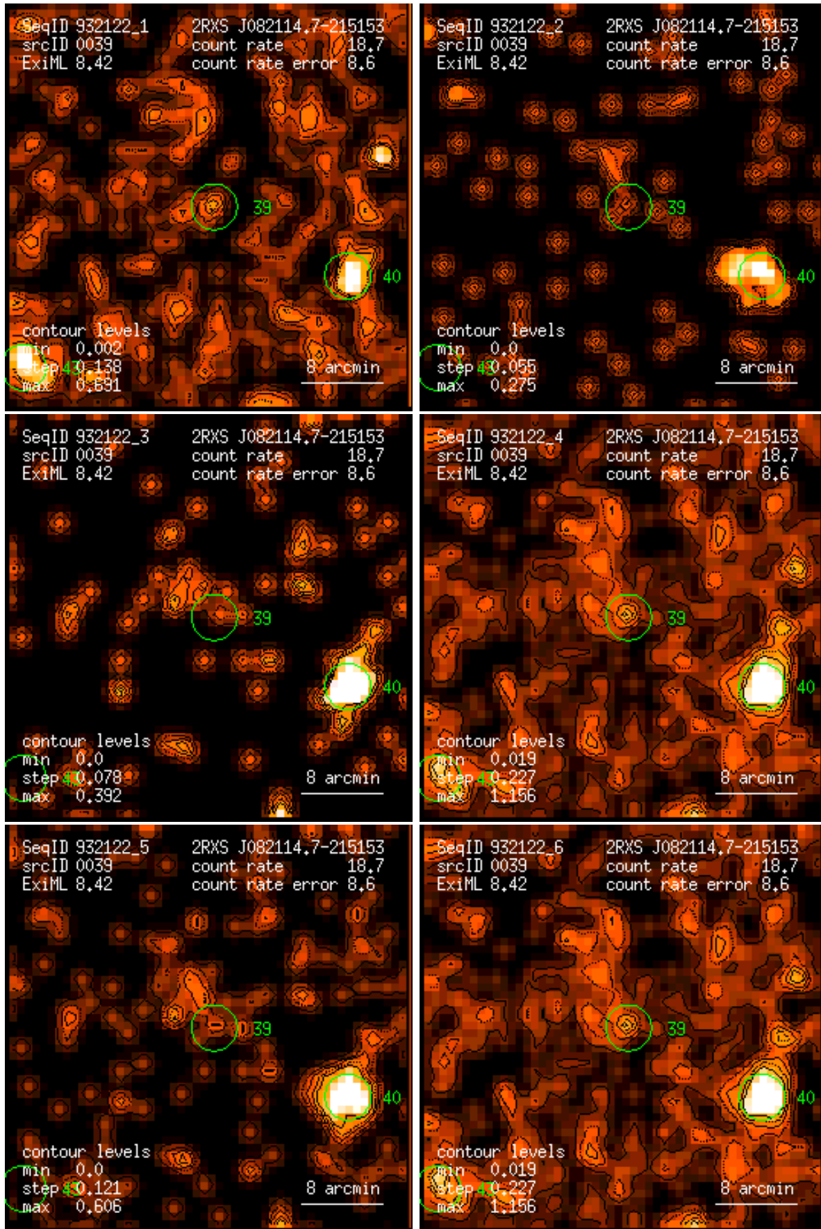
Figure 39: RASS 932122: detection 0039: band rate images, Gaussian filter: (1) PSPC channels 11 – 41, (2) 52 – 90, (3) 91 – 201, (4) 11 – 235, (5) 52 – 201, (6) 11 – 201. Broad band rates in counts/ks. Band rate contour levels in counts/ks/arcmin 2 .
