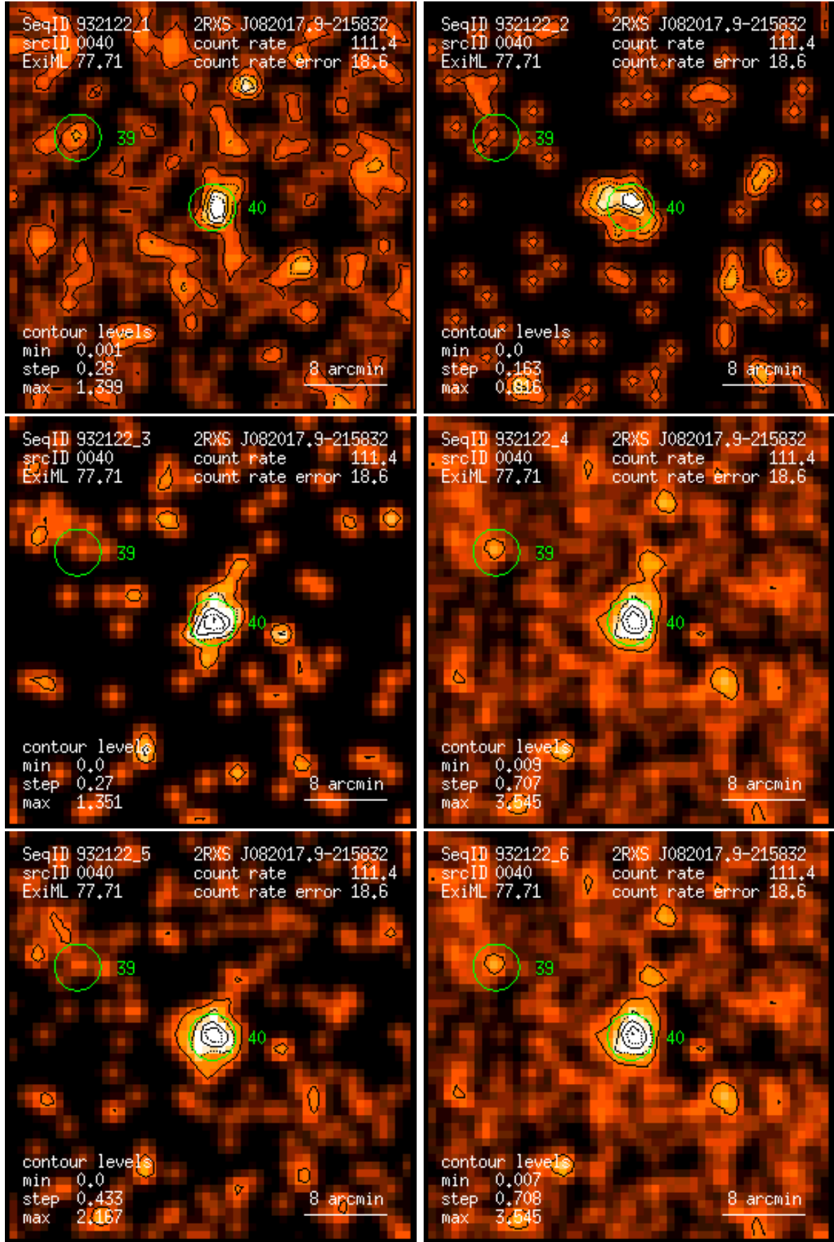
Figure 40: RASS 932122: detection 0040: band rate images, Gaussian filter: (1) PSPC channels 11 – 41, (2) 52 – 90, (3) 91 – 201, (4) 11 – 235, (5) 52 – 201, (6) 11 – 201. Broad band rates in counts/ks. Band rate contour levels in counts/ks/arcmin 2 .
