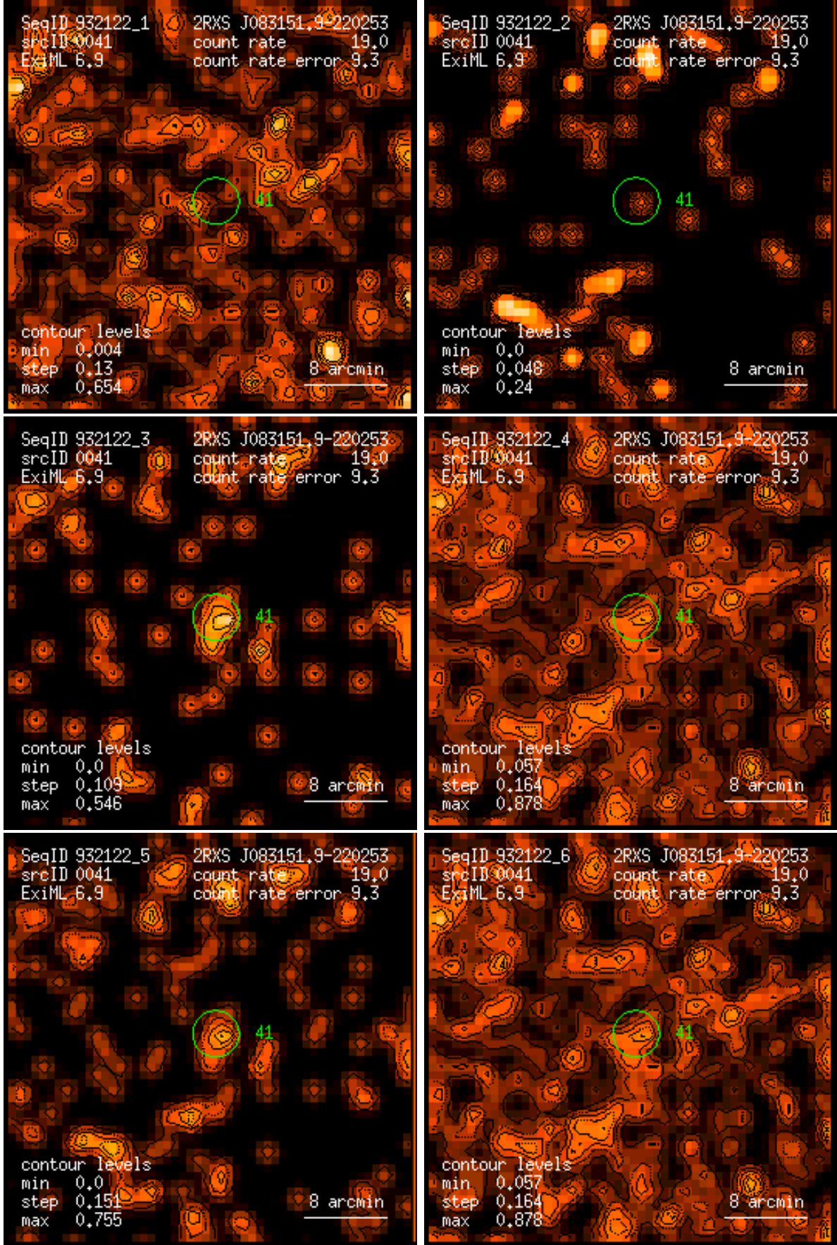
Figure 41: RASS 932122: detection 0041: band rate images, Gaussian filter: (1) PSPC channels 11 – 41, (2) 52 – 90, (3) 91 – 201, (4) 11 – 235, (5) 52 – 201, (6) 11 – 201. Broad band rates in counts/ks. Band rate contour levels in counts/ks/arcmin 2 .
