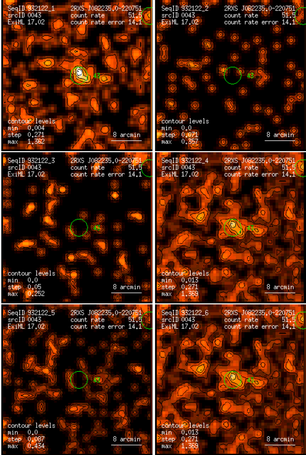
Figure 43: RASS 932122: detection 0043: band rate images, Gaussian filter: (1) PSPC channels 11 – 41, (2) 52 – 90, (3) 91 – 201, (4) 11 – 235, (5) 52 – 201, (6) 11 – 201. Broad band rates in counts/ks. Band rate contour levels in counts/ks/arcmin 2 .
