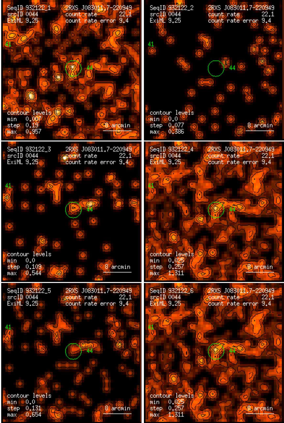
Figure 44: RASS 932122: detection 0044: band rate images, Gaussian filter: (1) PSPC channels 11 – 41, (2) 52 – 90, (3) 91 – 201, (4) 11 – 235, (5) 52 – 201, (6) 11 – 201. Broad band rates in counts/ks. Band rate contour levels in counts/ks/arcmin 2 .
