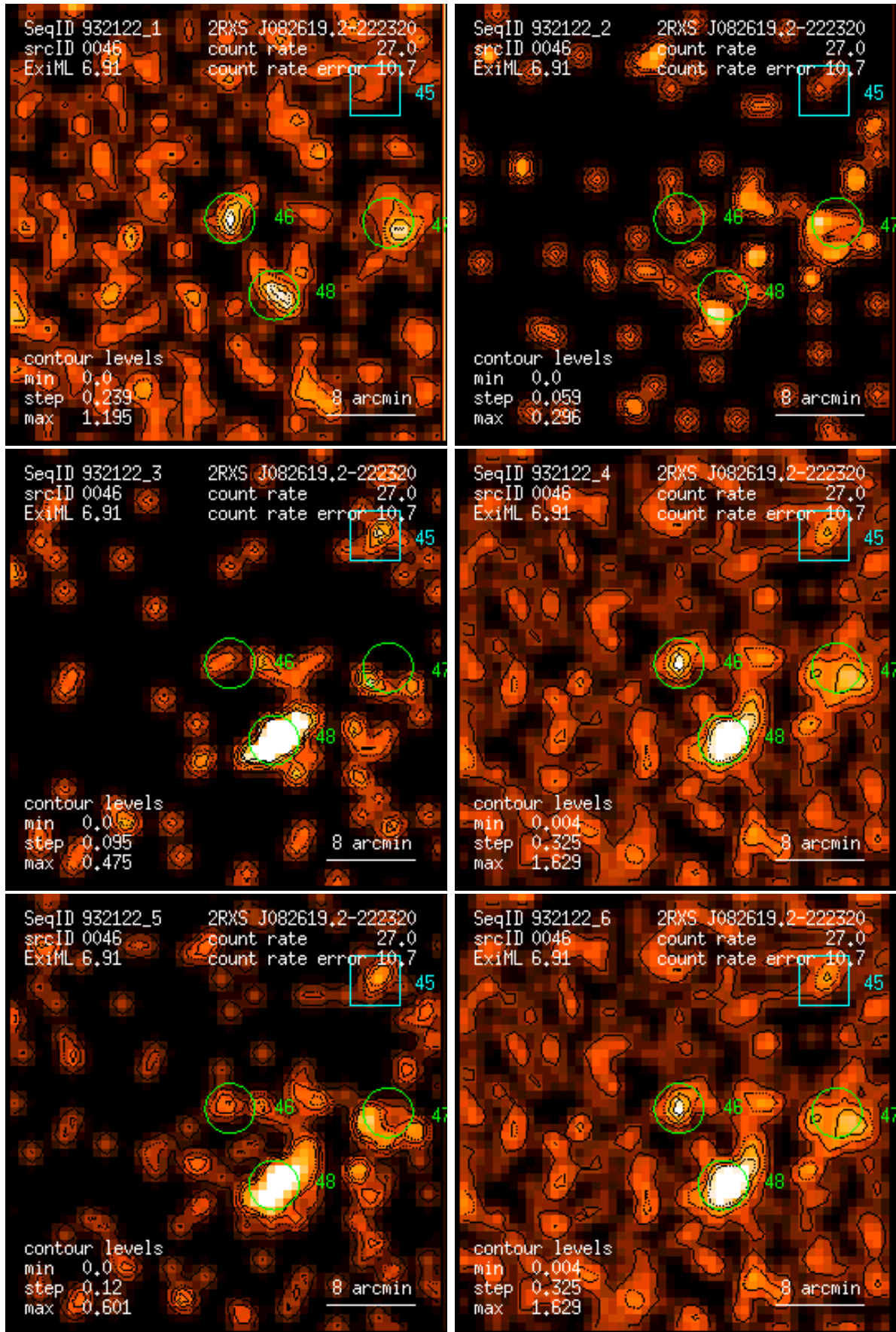
Figure 46: RASS 932122: detection 0046: band rate images, Gaussian filter: (1) PSPC channels 11 – 41, (2) 52 – 90, (3) 91 – 201, (4) 11 – 235, (5) 52 – 201, (6) 11 – 201. Broad band rates in counts/ks. Band rate contour levels in counts/ks/arcmin 2 .
