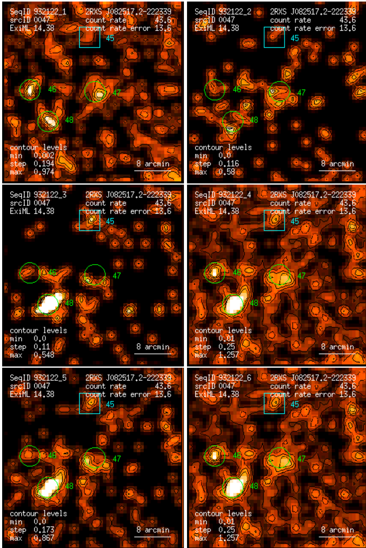
Figure 47: RASS 932122: detection 0047: band rate images, Gaussian filter: (1) PSPC channels 11 – 41, (2) 52 – 90, (3) 91 – 201, (4) 11 – 235, (5) 52 – 201, (6) 11 – 201. Broad band rates in counts/ks. Band rate contour levels in counts/ks/arcmin 2 .
