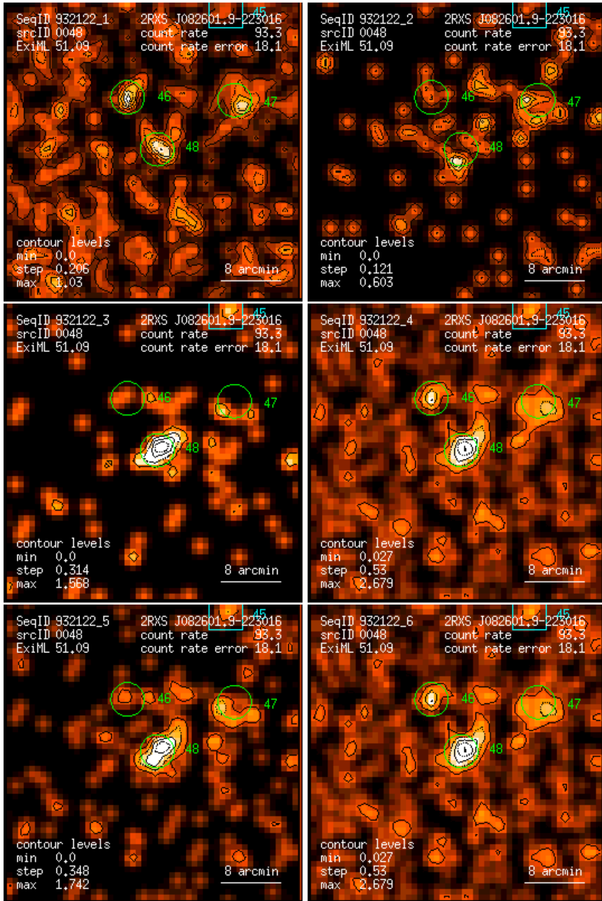
Figure 48: RASS 932122: detection 0048: band rate images, Gaussian filter: (1) PSPC channels 11 – 41, (2) 52 – 90, (3) 91 – 201, (4) 11 – 235, (5) 52 – 201, (6) 11 – 201. Broad band rates in counts/ks. Band rate contour levels in counts/ks/arcmin 2 .
