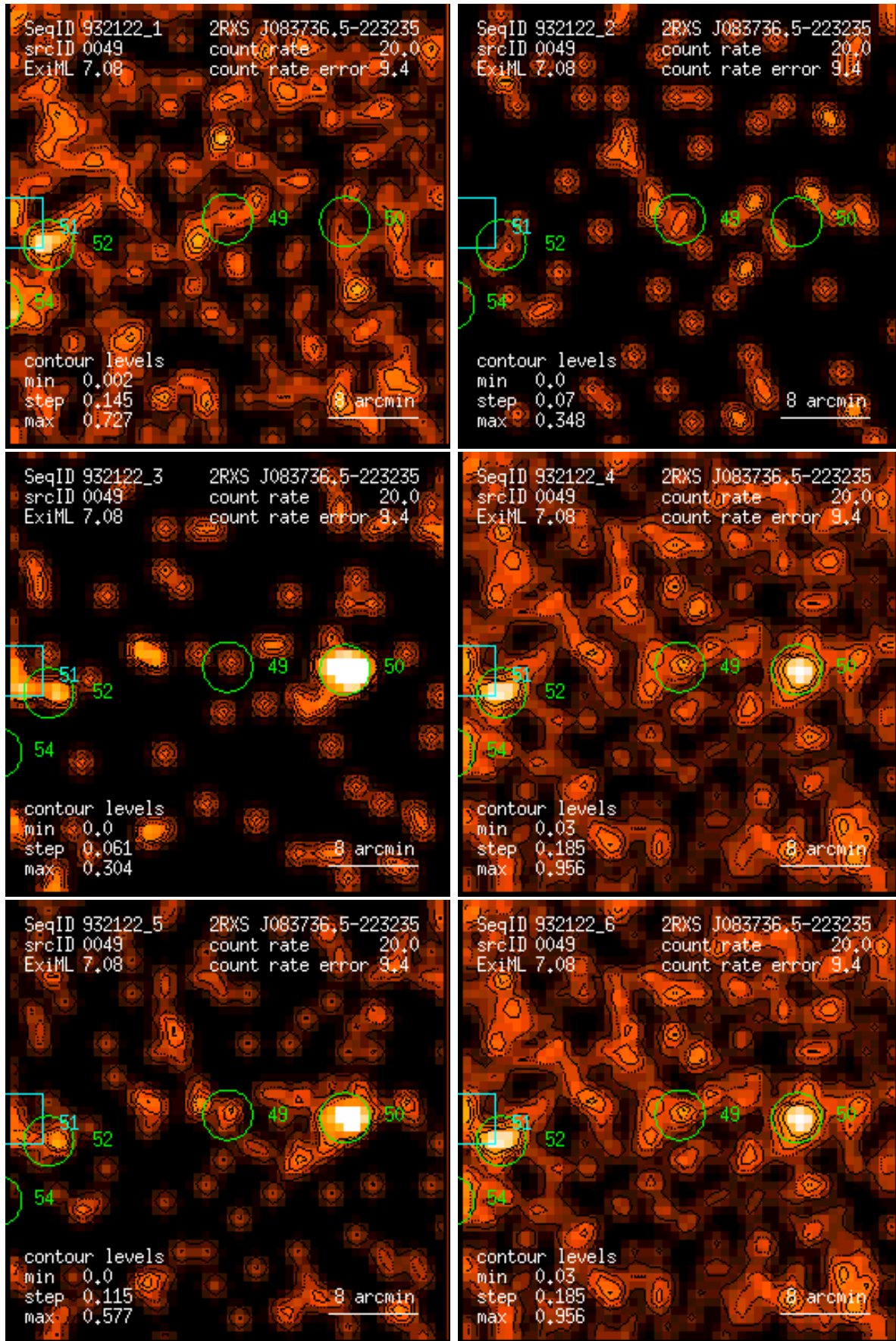
Figure 49: RASS 932122: detection 0049: band rate images, Gaussian filter: (1) PSPC channels 11 – 41, (2) 52 – 90, (3) 91 – 201, (4) 11 – 235, (5) 52 – 201, (6) 11 – 201. Broad band rates in counts/ks. Band rate contour levels in counts/ks/arcmin 2 .
