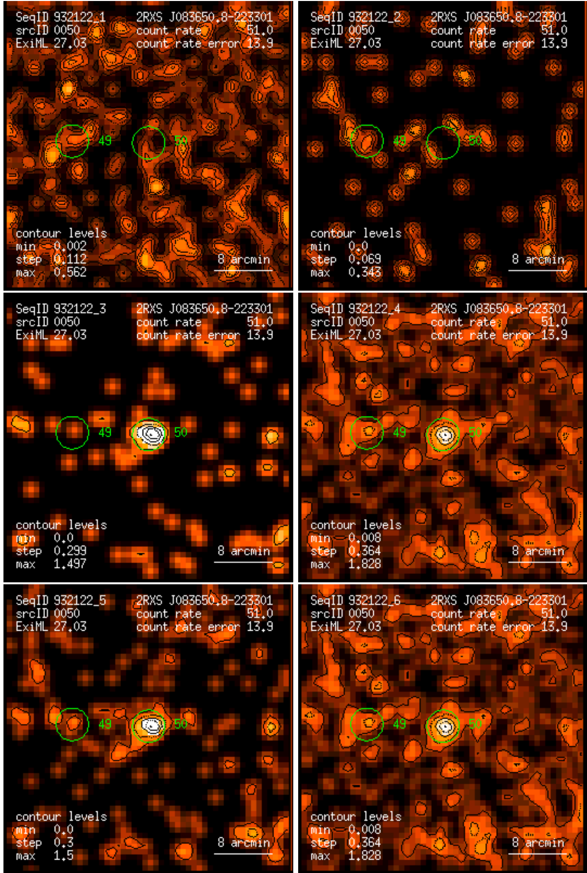
Figure 50: RASS 932122: detection 0050: band rate images, Gaussian filter: (1) PSPC channels 11 – 41, (2) 52 – 90, (3) 91 – 201, (4) 11 – 235, (5) 52 – 201, (6) 11 – 201. Broad band rates in counts/ks. Band rate contour levels in counts/ks/arcmin 2 .
