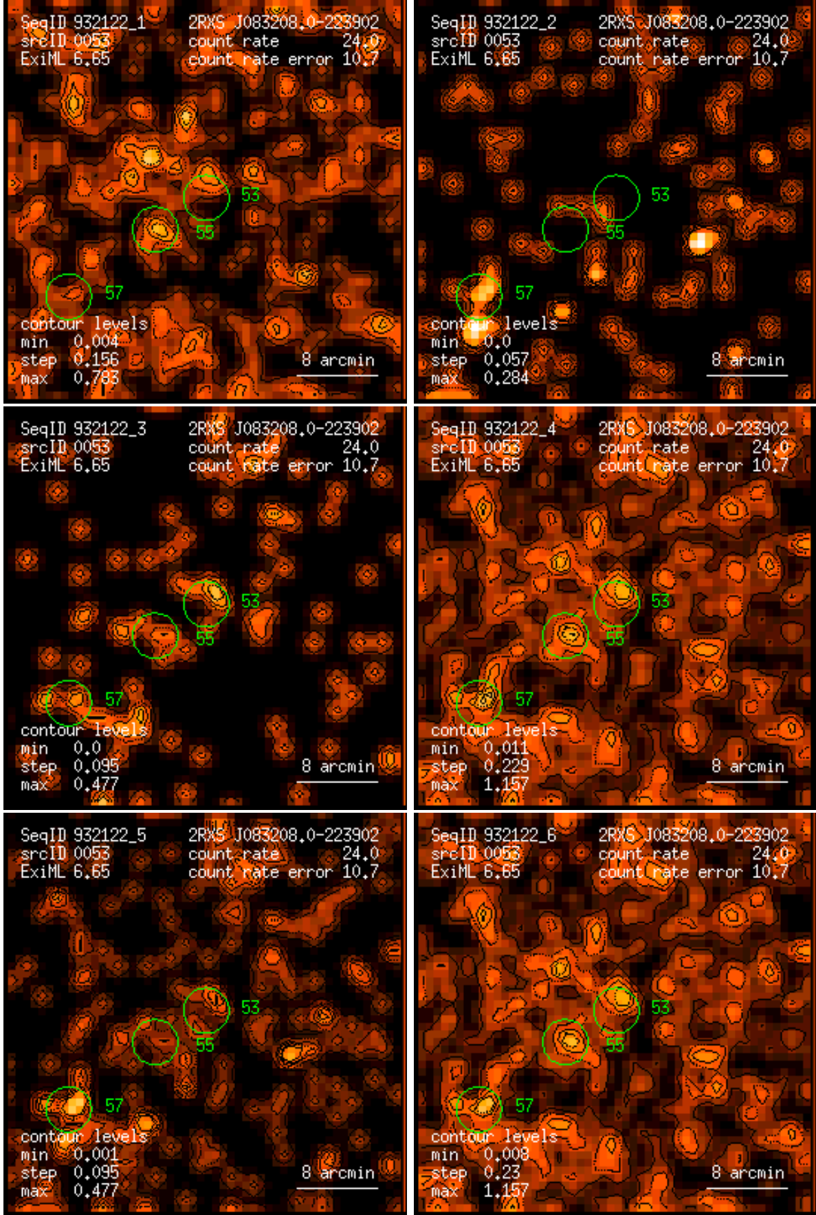
Figure 53: RASS 932122: detection 0053: band rate images, Gaussian filter: (1) PSPC channels 11 – 41, (2) 52 – 90, (3) 91 – 201, (4) 11 – 235, (5) 52 – 201, (6) 11 – 201. Broad band rates in counts/ks. Band rate contour levels in counts/ks/arcmin 2 .
