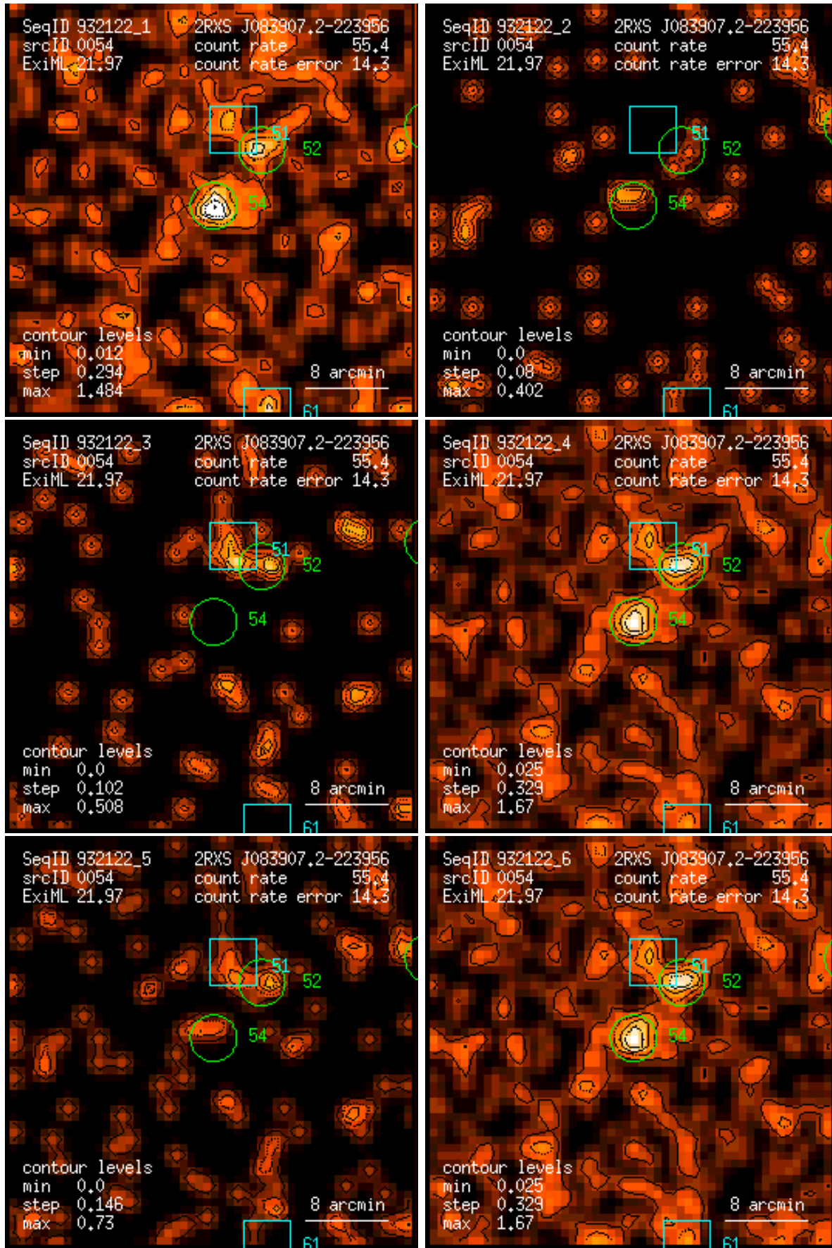
Figure 54: RASS 932122: detection 0054: band rate images, Gaussian filter: (1) PSPC channels 11 – 41, (2) 52 – 90, (3) 91 – 201, (4) 11 – 235, (5) 52 – 201, (6) 11 – 201. Broad band rates in counts/ks. Band rate contour levels in counts/ks/arcmin 2 .
