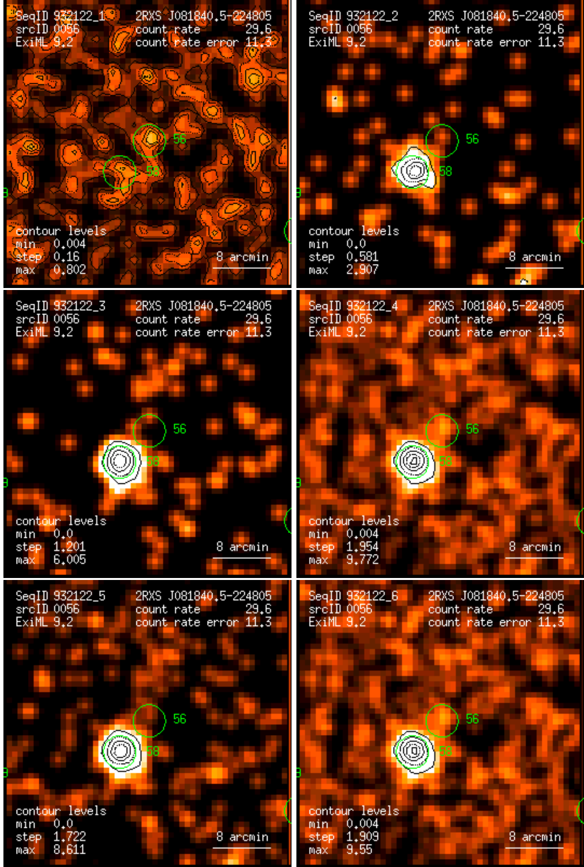
Figure 56: RASS 932122: detection 0056: band rate images, Gaussian filter: (1) PSPC channels 11 – 41, (2) 52 – 90, (3) 91 – 201, (4) 11 – 235, (5) 52 – 201, (6) 11 – 201. Broad band rates in counts/ks. Band rate contour levels in counts/ks/arcmin 2 .
